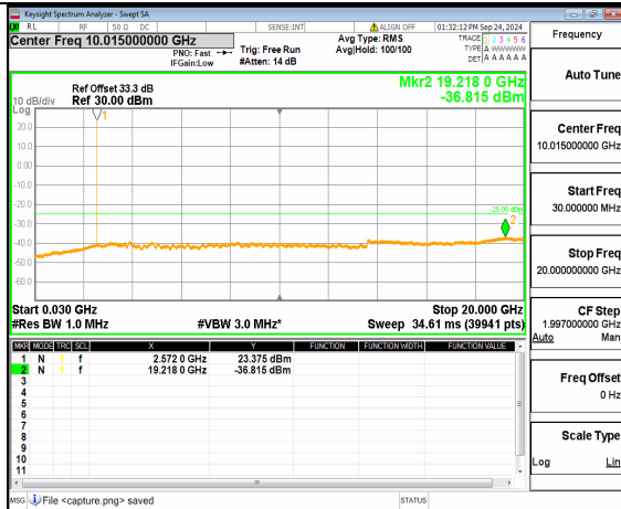
n38 (30MHz-20GHz) 40M DFT-s-OFDM QPSK Inner 1RB Left Low
