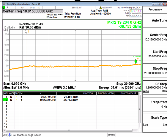
n38 (30MHz-20GHz) 40M DFT-s-OFDM BPSK Inner 1RB Left Mid
