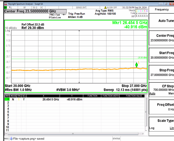
n38 (20GHz-27GHz) 40M DFT-s-OFDM QPSK Inner 1RB Left Low
