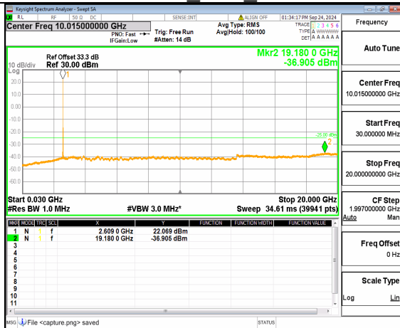
n38 (30MHz-20GHz) 40M DFT-s-OFDM QPSK Inner 1RB Right Low
