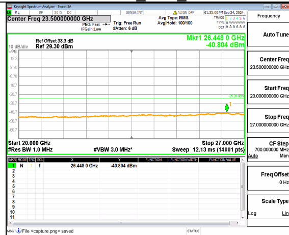
n38 (20GHz-27GHz) 40M DFT-s-OFDM QPSK Inner 1RB Right Low
