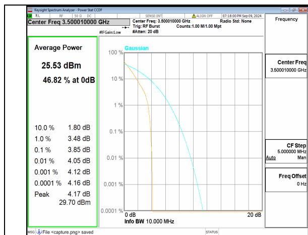
n78(3450-3550MHz) 10M DFT-s-OFDM BPSK Outer_Full Mid
