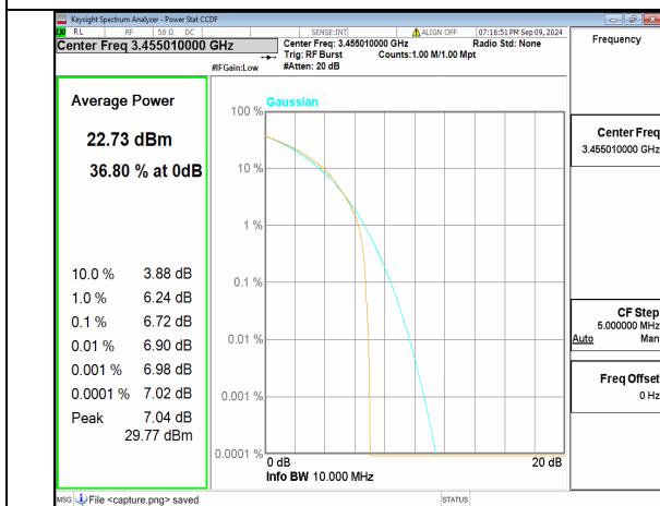
n78(3450-3550MHz) 10M CP-OFDM QPSK Outer_Full Low
