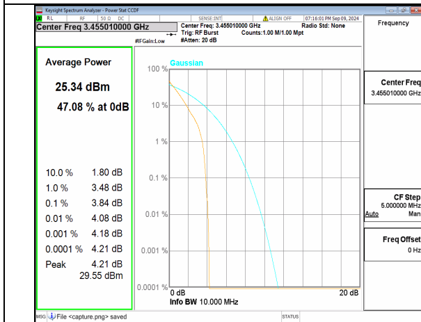
n78(3450-3550MHz) 10M DFT-s-OFDM BPSK Outer_Full Low
