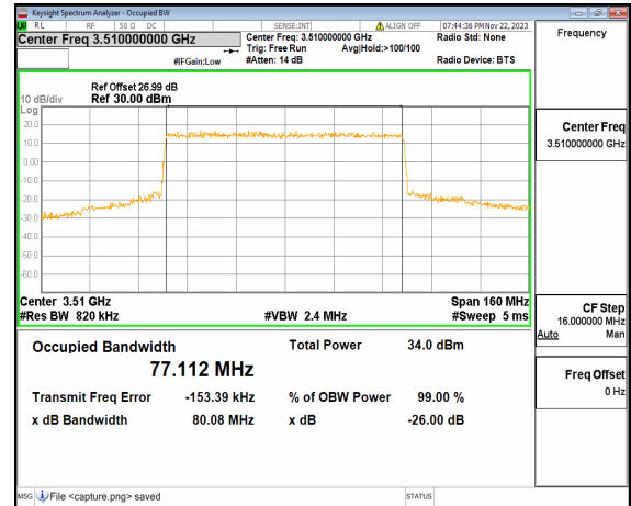
n77(3450-3550MHz) 80M DFT-s-OFDM QPSK Outer_Full High
