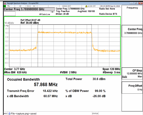
n78(3700-3800MHz) 60M DFT-s-OFDM 64QAM Outer_Full High
