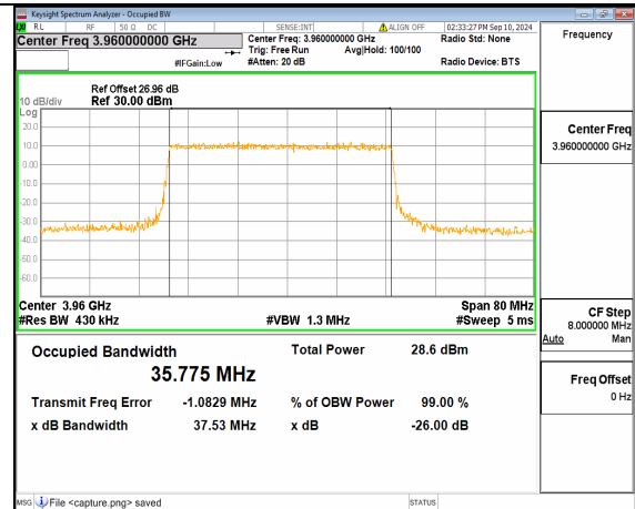
n77(3700-3980MHz) 40M DFT-s-OFDM 64QAM Outer_Full High
