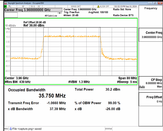
n77(3700-3980MHz) 40M DFT-s-OFDM QPSK Outer_Full High
