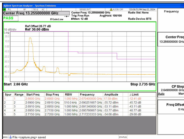
41C / 5+20MHz / High CH / QPSK / 1#24-1#0
