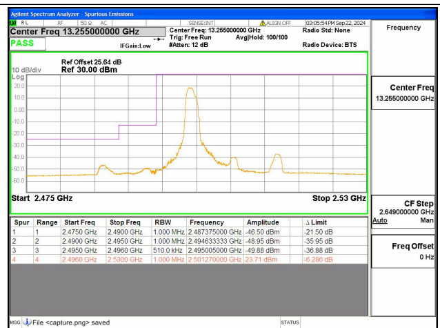
41C / 5+20MHz / Low CH / QPSK / 1#24-1#0
