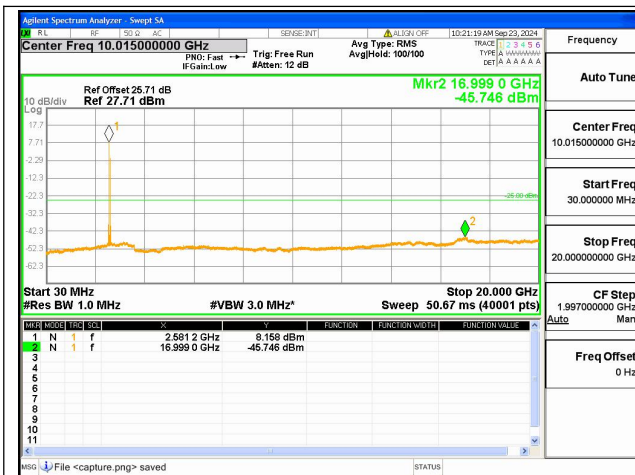
38C-30M-20G / 20+20MHz / QPSK / High CH / 1@0-1@99
