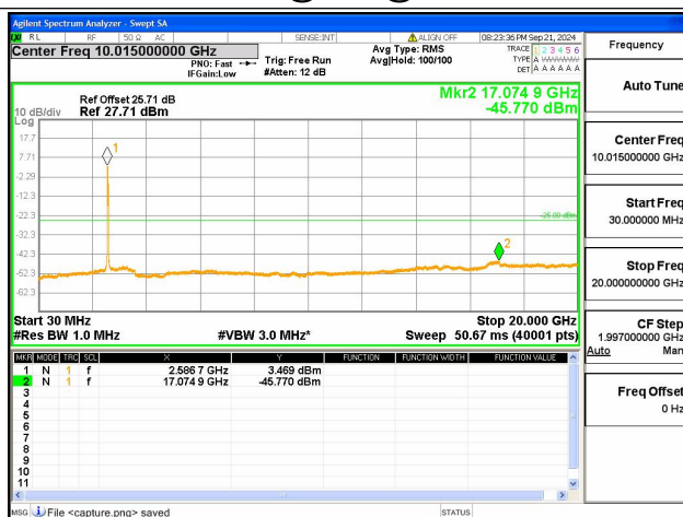
38C-30M-20G / 20+20MHz / QPSK / High CH / 100@0-100@0
