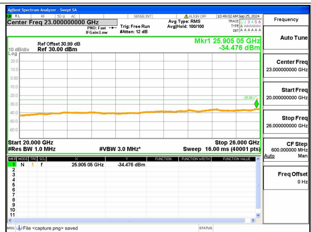
7A-12A-20G-26G / 20+10MHz / QPSK / High+Low CH / 1@0-1@49
