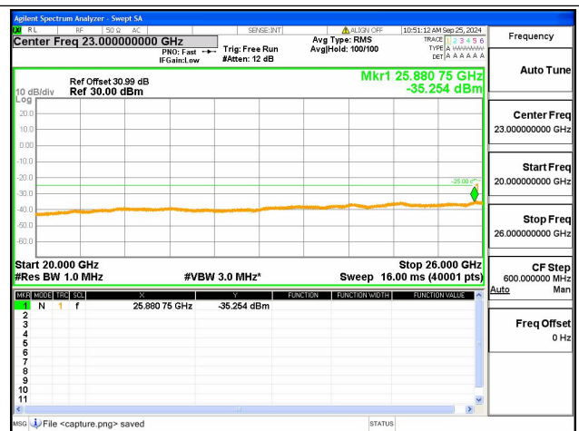
7A-12A-20G-26G / 20+10MHz / QPSK / High+Mid CH / 1@0-1@49
