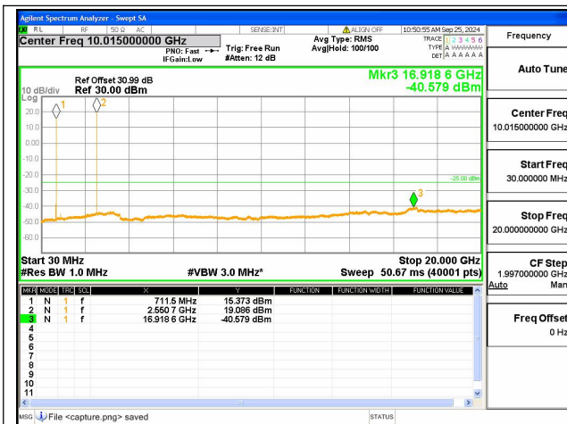
7A-12A-30M-20G / 20+10MHz / QPSK / High+Mid CH / 1@0-1@49
