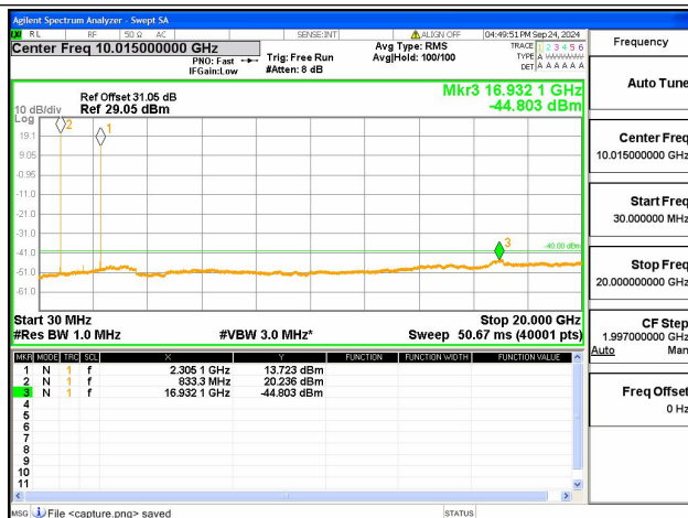
5A-30A-30M-20G / 10+10MHz / QPSK / Low+Low CH / 1@49-1@0
