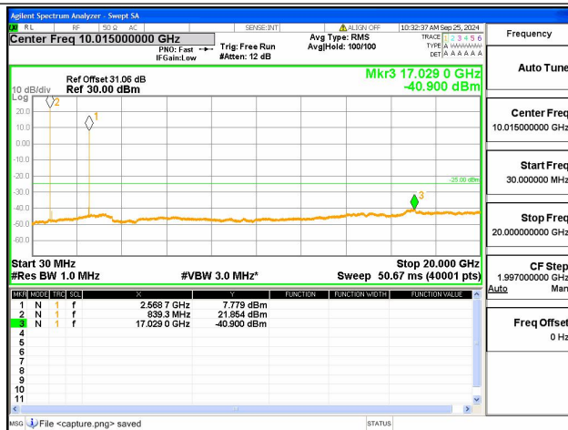
5A-7A-30M-20G / 10+20MHz / QPSK / High+High CH / 1@0-1@99
