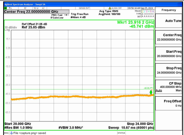
5A-30A-20G-24G / 10+10MHz / QPSK / Low+Low CH / 1@0-1@49
