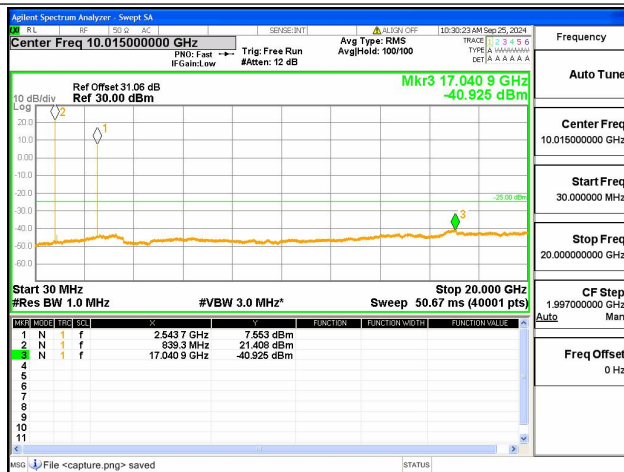
5A-7A-30M-20G / 10+20MHz / QPSK / High+Mid CH / 1@0-1@99
