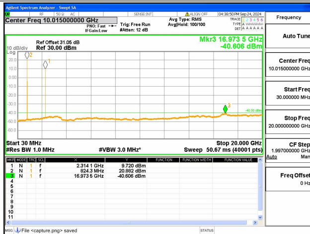
5A-30A-30M-20G / 10+10MHz / QPSK / Low+Low CH / 1@0-1@49
