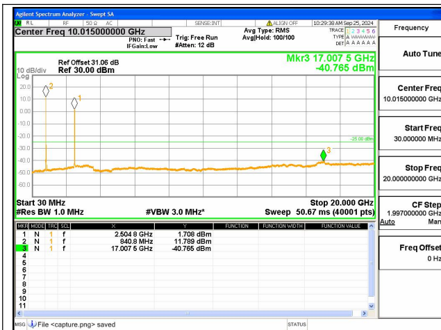
5A-7A-30M-20G / 10+20MHz / QPSK / High+Low CH / 50@0-100@0
