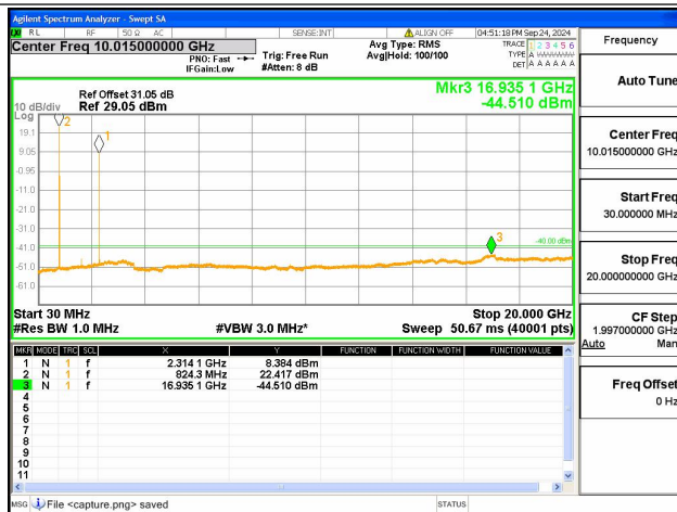
5A-30A-30M-20G / 10+10MHz / QPSK / Low+Mid CH / 1@0-1@49
