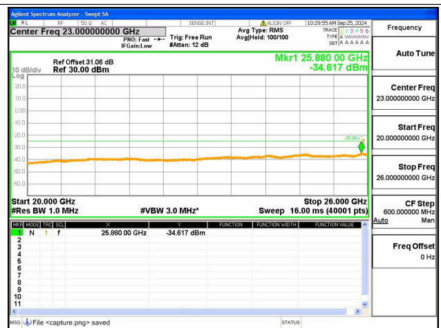
5A-7A-20G-26G / 10+20MHz / QPSK / High+Low CH / 50@0-100@0
