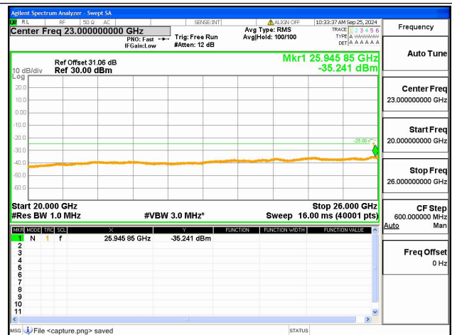
5A-7A-20G-26G / 10+20MHz / QPSK / High+High CH / 1@49-1@0
