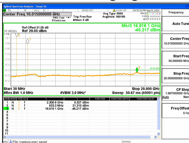
5A-30A-30M-20G / 10+10MHz / QPSK / Low+Mid CH / 1@49-1@0
