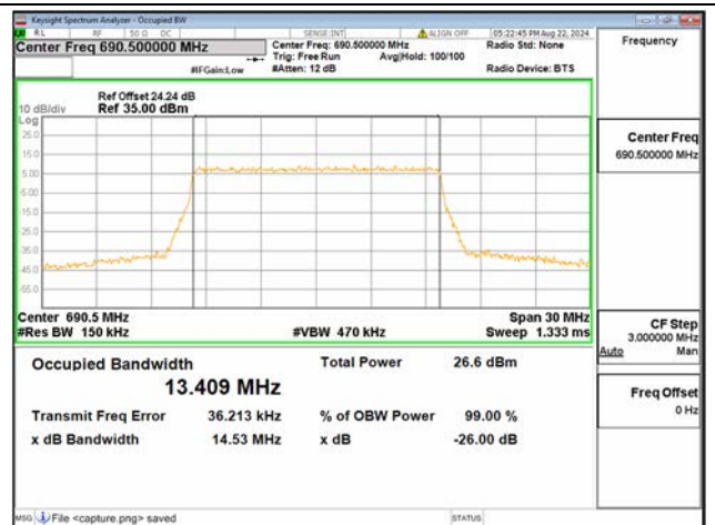
B71 / 15MHz / 256QAM/ High CH
