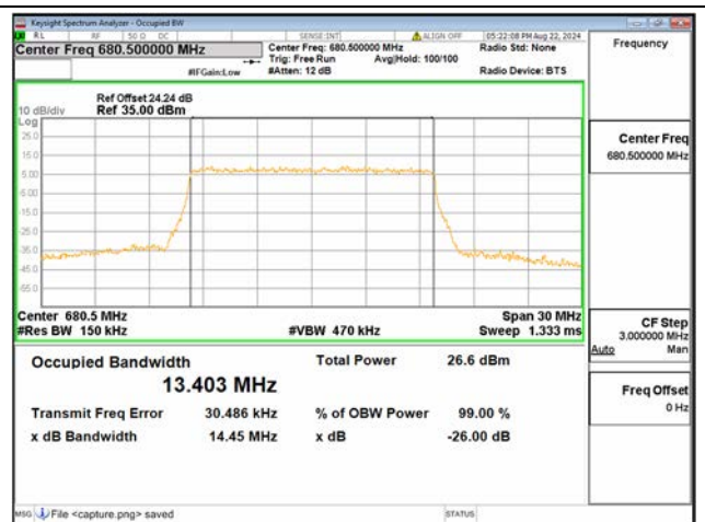
B71 / 15MHz / 256QAM/ Mid CH
