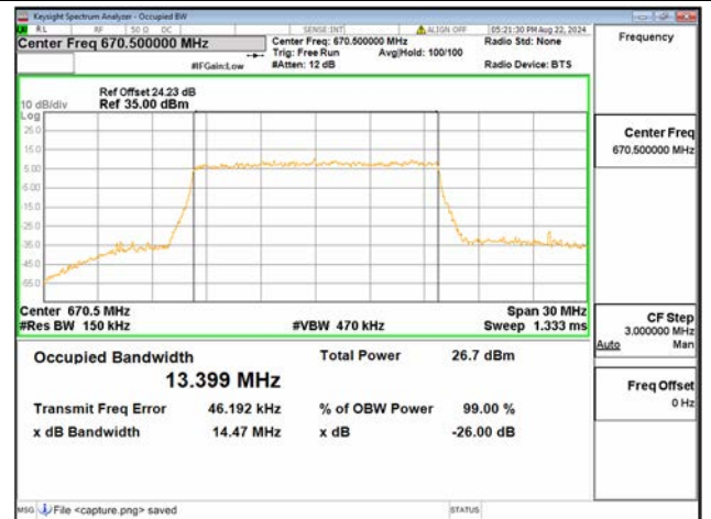
B71 / 15MHz / 256QAM/ Low CH
