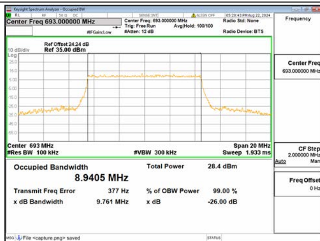
B71 / 10MHz / 64QAM/ High CH
