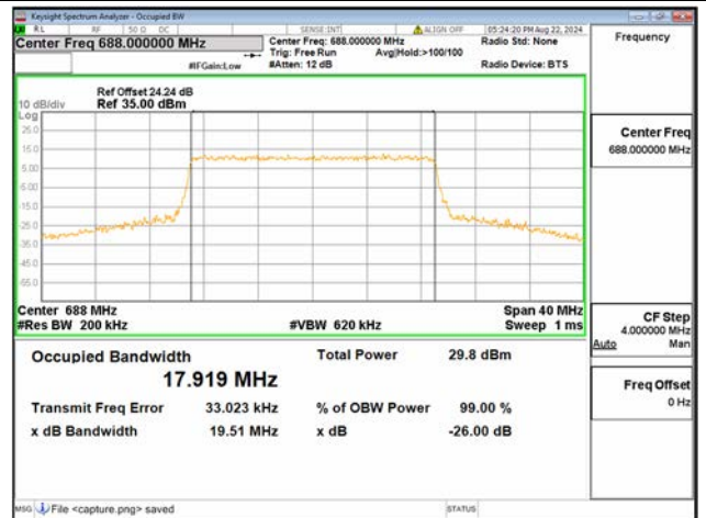
B71 / 20MHz / 16QAM/ High CH
