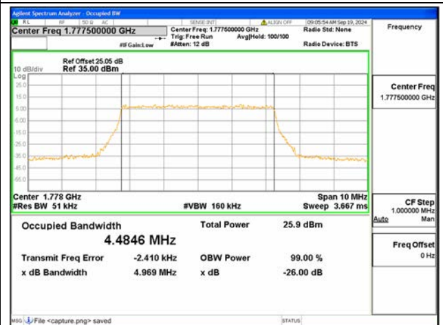
B66 / 5MHz / 256QAM/ High CH
