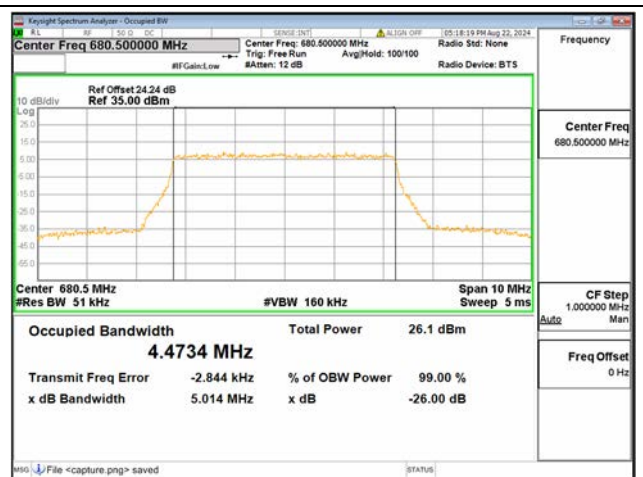
B71 / 5MHz / 256QAM/ Mid CH
