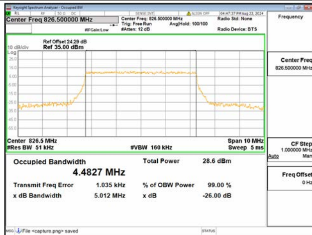
B26 Part22 / 5MHz / 64QAM/ Low CH
