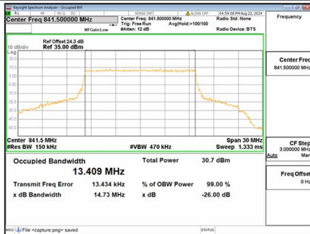
B26 Part22 / 15MHz / QPSK/ High CH
