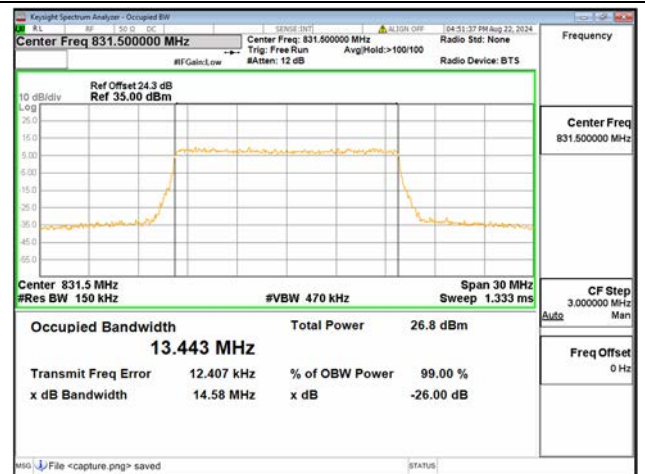
B26 Part22 / 15MHz / 256QAM/ Low CH
