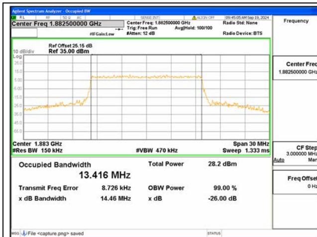
B25 / 15MHz / 64QAM/ Mid CH
