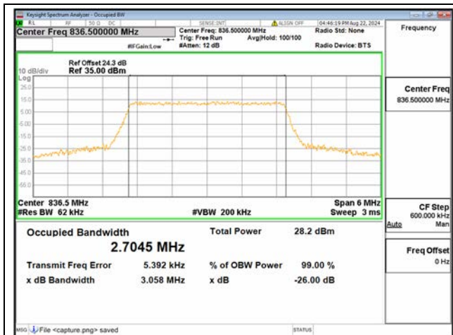
B26 Part22 / 3MHz / 64QAM/ Mid CH
