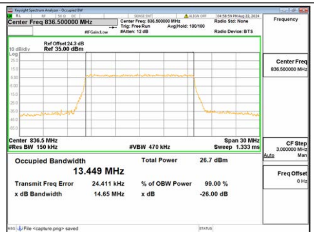
B26 Part22 / 15MHz / 256QAM/ Mid CH
