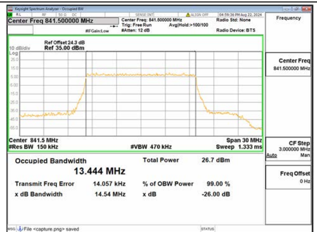
B26 Part22 / 15MHz / 256QAM/ High CH
