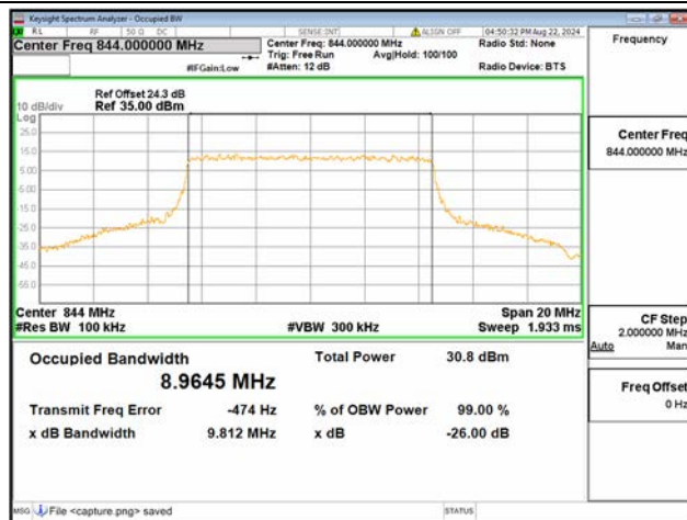
B26 Part22 / 10MHz / QPSK/ High CH
