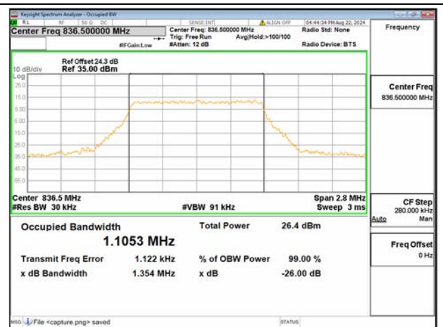
B26 Part22 / 1.4MHz / 256QAM/ Mid CH
