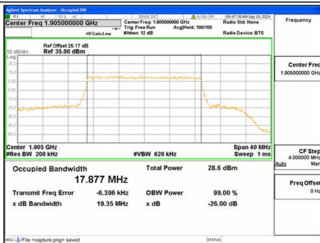
B25 / 20MHz / 64QAM/ High CH
