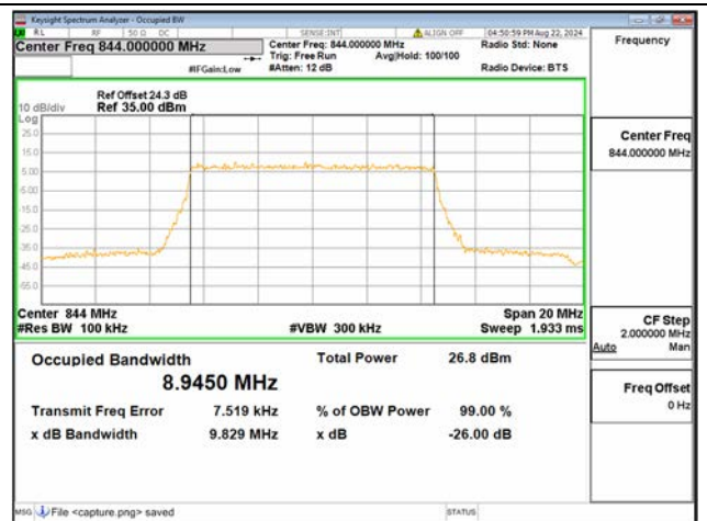
B26 Part22 / 10MHz / 256QAM/ High CH
