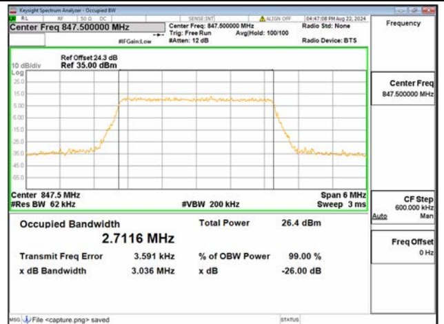
B26 Part22 / 3MHz / 256QAM/ High CH
