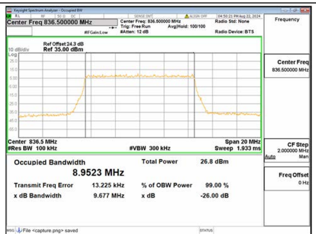
B26 Part22 / 10MHz / 256QAM/ Mid CH
