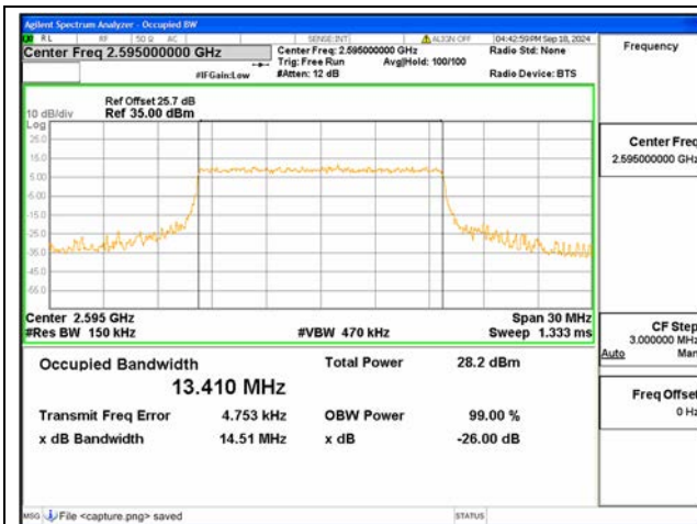
B38 / 15MHz / 64QAM/ Mid CH
