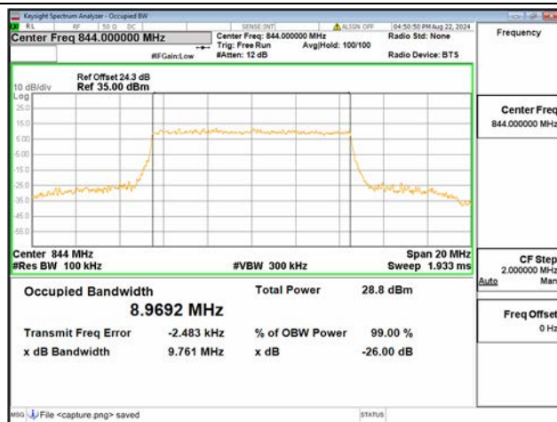
B26 Part22 / 10MHz / 64QAM/ High CH
