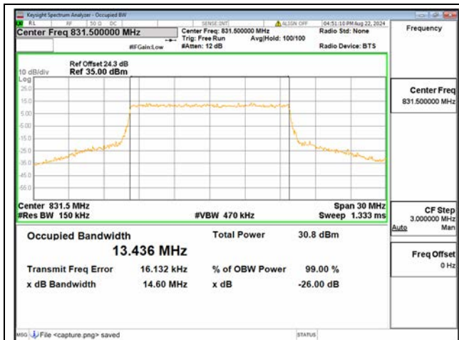
B26 Part22 / 15MHz / QPSK/ Low CH
