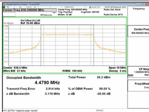
B26 Part22 / 5MHz / QPSK/ Mid CH
