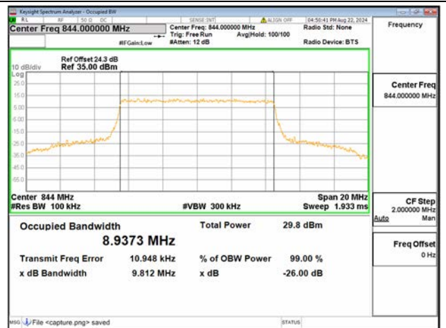
B26 Part22 / 10MHz / 16QAM/ High CH
