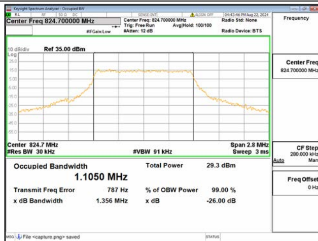
B26 Part22 / 1.4MHz / 64QAM/ Low CH
