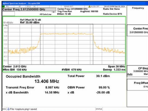
B38 / 15MHz / QPSK/ High CH
