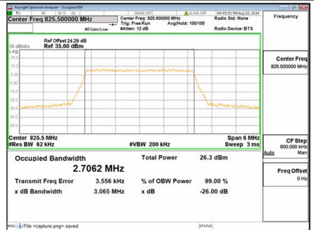
B26 Part22 / 3MHz / 256QAM/ Low CH
