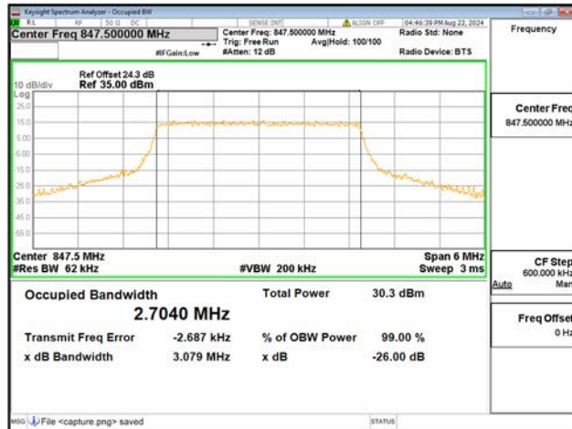
B26 Part22 / 3MHz / QPSK/ High CH
