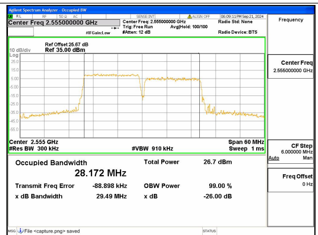
7C / 15+15MHz / 256QAM/ High CH
