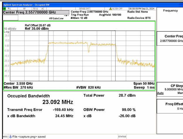
7C / 15+10MHz / 64QAM/ High CH
