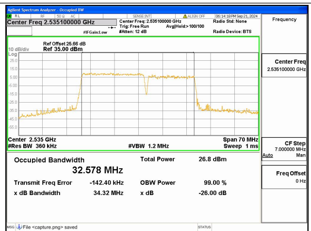
7C / 20+15MHz / 256QAM/ Mid CH
