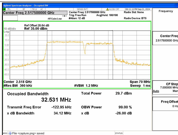
7C / 20+15MHz / QPSK/ Low CH
