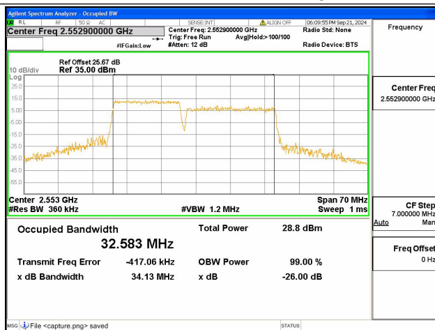
7C / 15+20MHz / 64QAM/ High CH
