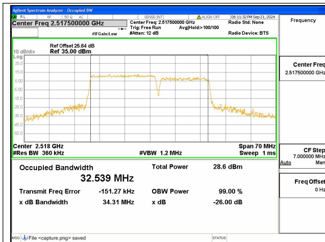
7C / 20+15MHz / 64QAM/ Low CH
