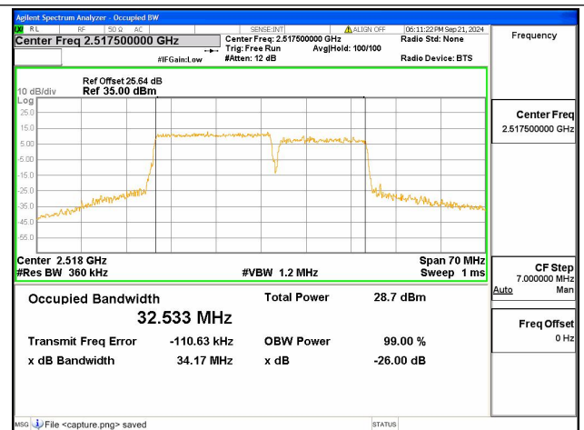
7C / 20+15MHz / 16QAM/ Low CH
