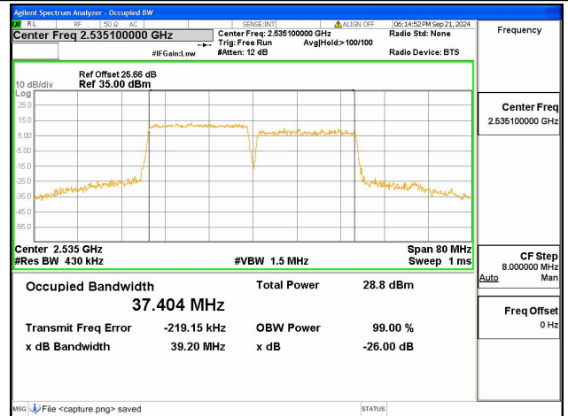
7C / 20+20MHz / 16QAM/ Mid CH
