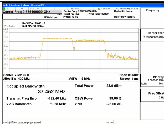
7C / 20+20MHz / 64QAM/ Mid CH
