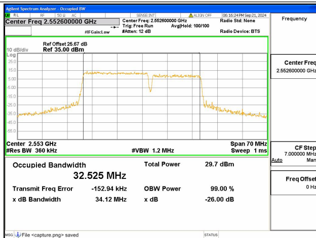
7C / 20+15MHz / QPSK/ High CH
