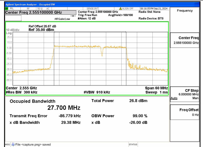
7C / 20+10MHz / 256QAM/ High CH
