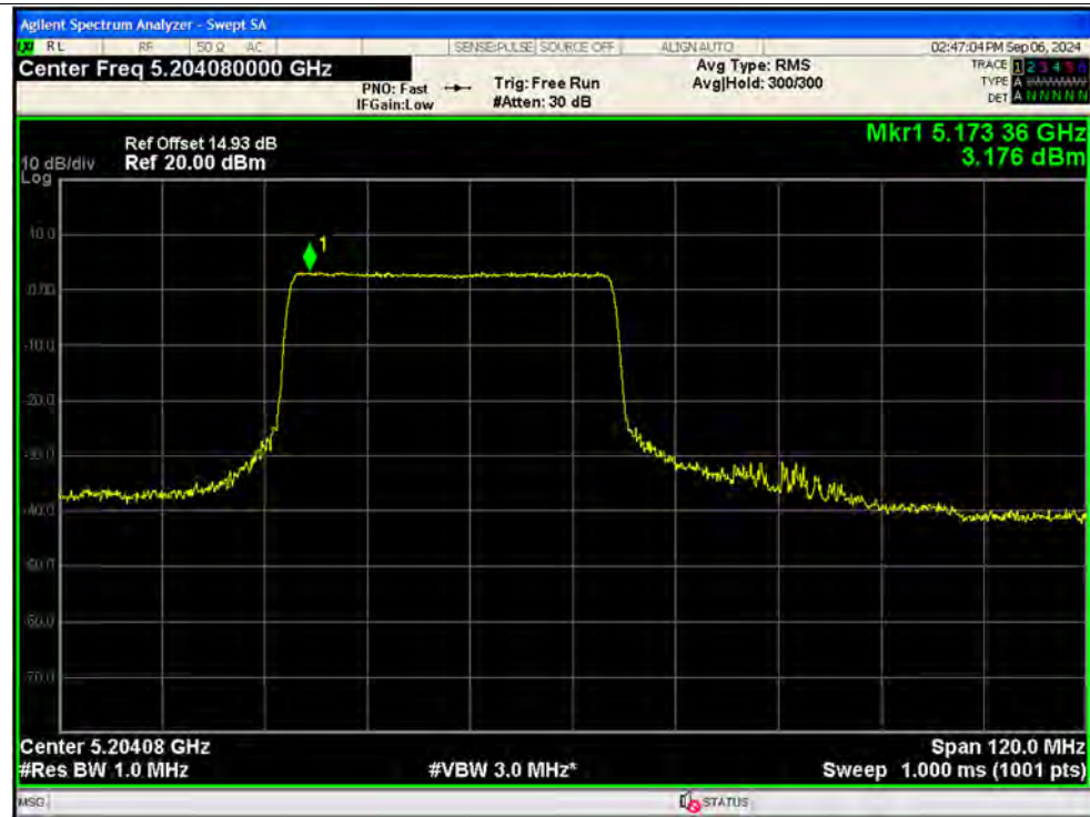
PSD NVNT ax80 484@65 5210MHz Ant13 SISO
