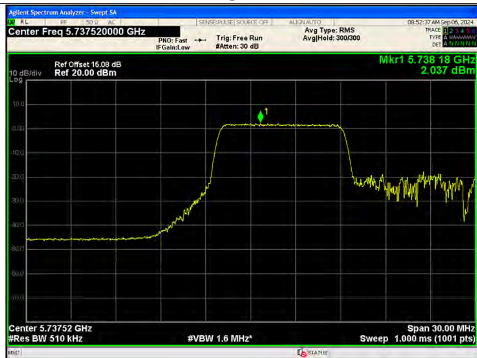
PSD NVNT ax20 106@53 5745MHz Ant13 SISO
