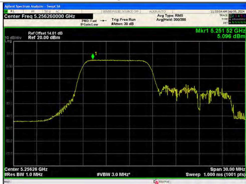
PSD NVNT ax20 106@53 5260MHz Ant13 MIMO
