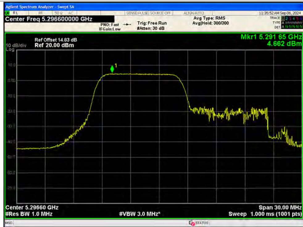
PSD NVNT ax20 106@53 5300MHz Ant13 MIMO
