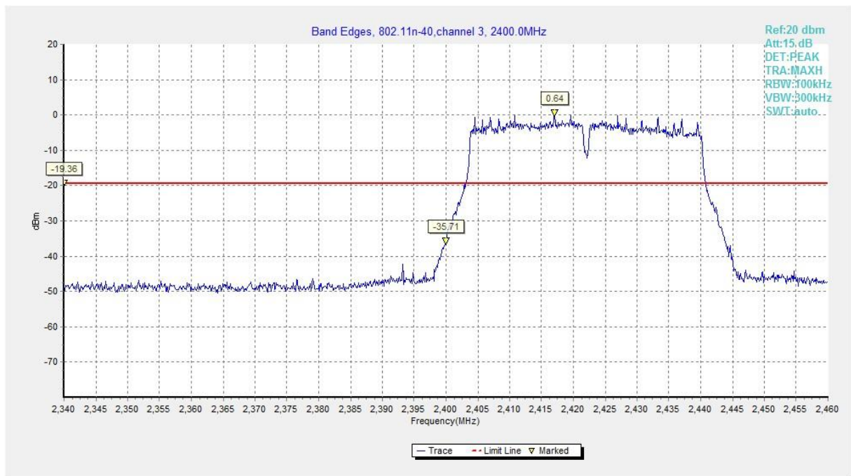
Fig.B.5.7 Band Edges (802.11n-HT40, Ch 3)
