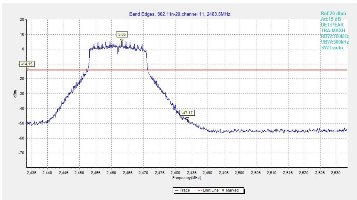
Fig.B.5.6 Band Edges (802.11n-HT20, Ch 11)
