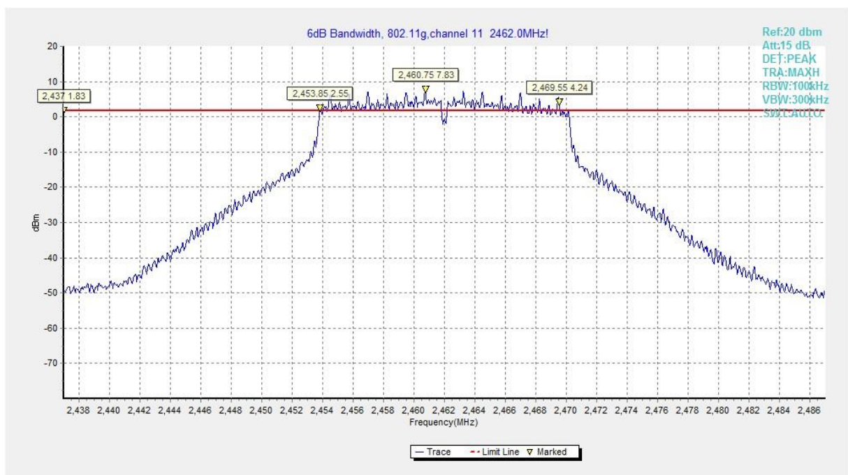
Fig.B.4.6 Occupied 6dB Bandwidth (802.11g, Ch 11)
