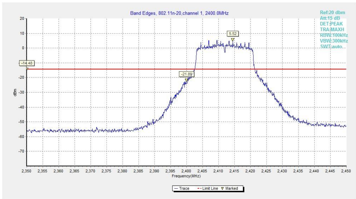
Fig.B.5.5 Band Edges (802.11n-HT20, Ch 1)
