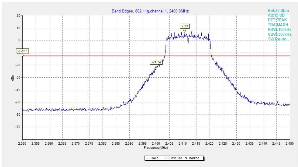
Fig.B.5.3 Band Edges (802.11g, Ch 1)
