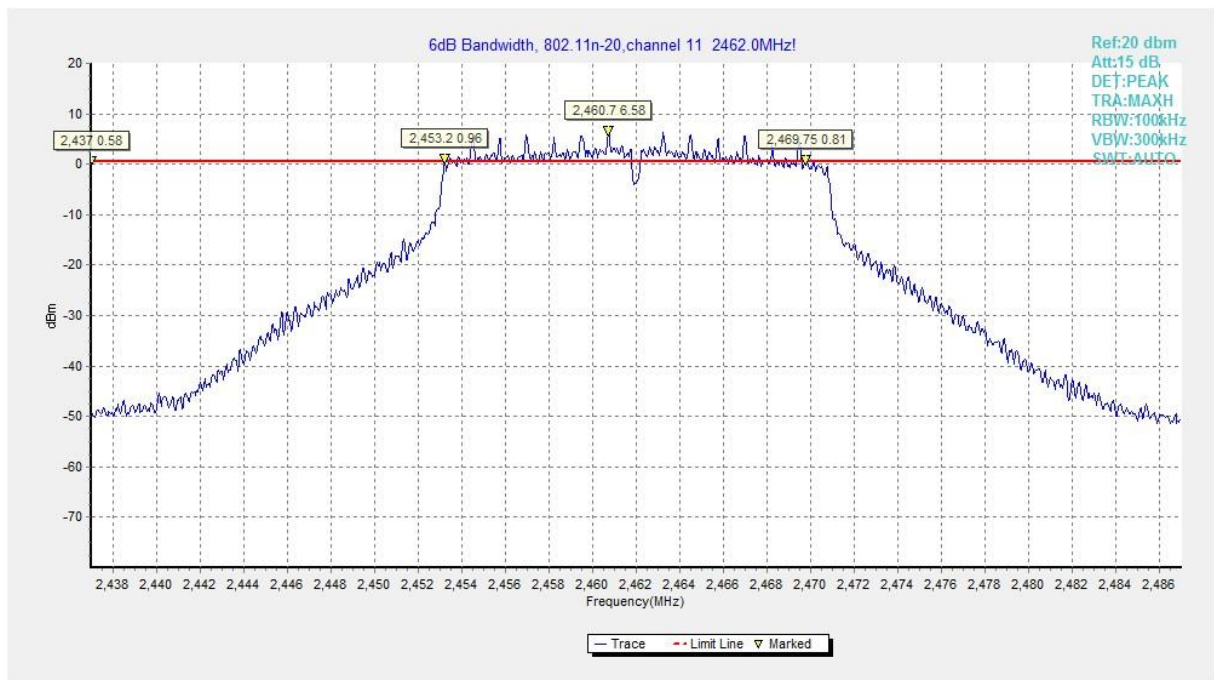
Fig.B.4.9 Occupied 6dB Bandwidth (802.11n-HT20, Ch 11)
