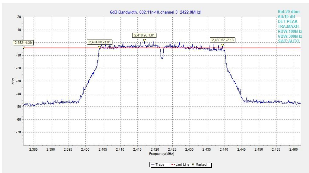
Fig.B.4.10 Occupied 6dB Bandwidth (802.11n-40MHz, Ch 3)
