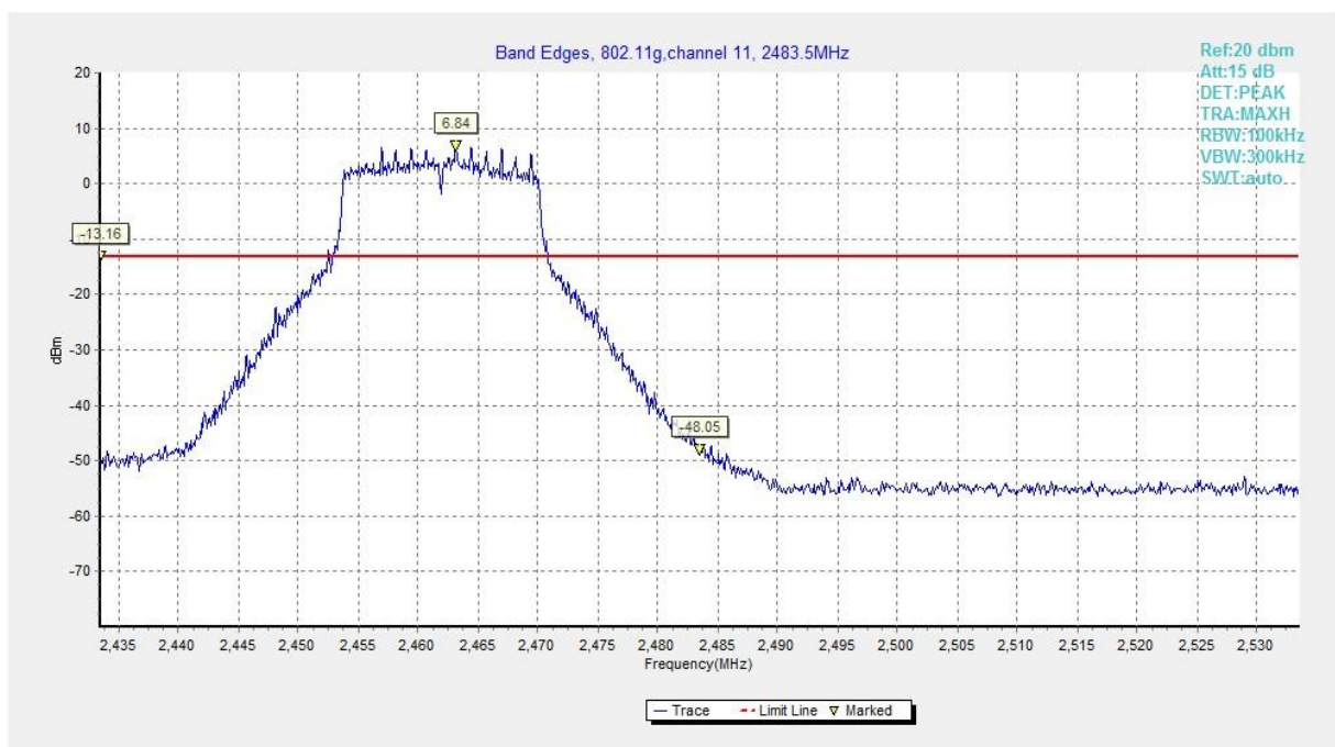
Fig.B.5.4 Band Edges (802.11g, Ch 11)
