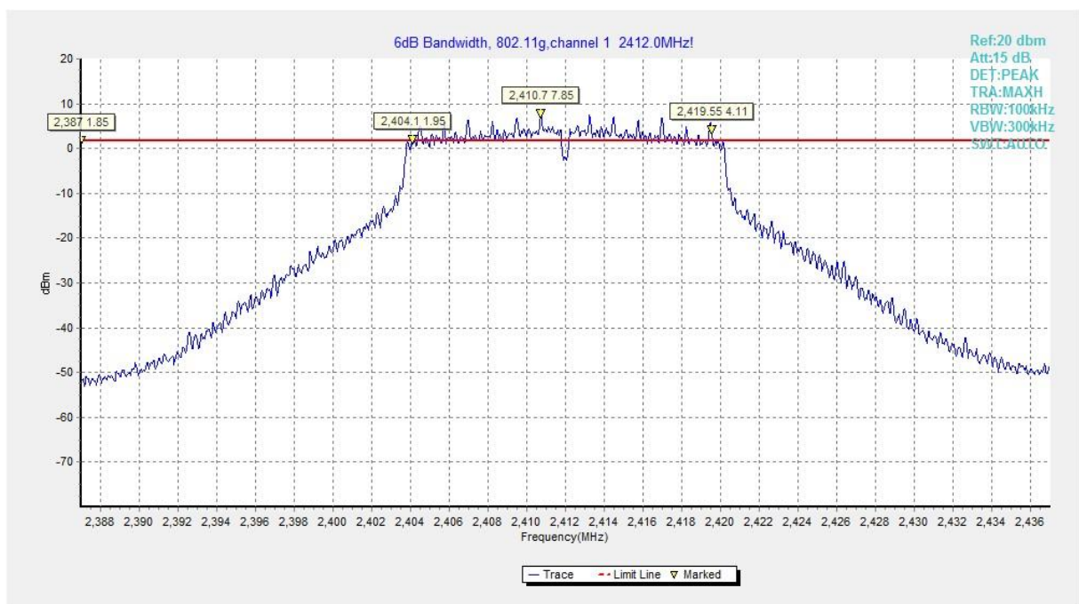
Fig.B.4.4 Occupied 6dB Bandwidth (802.11g, Ch 1)
