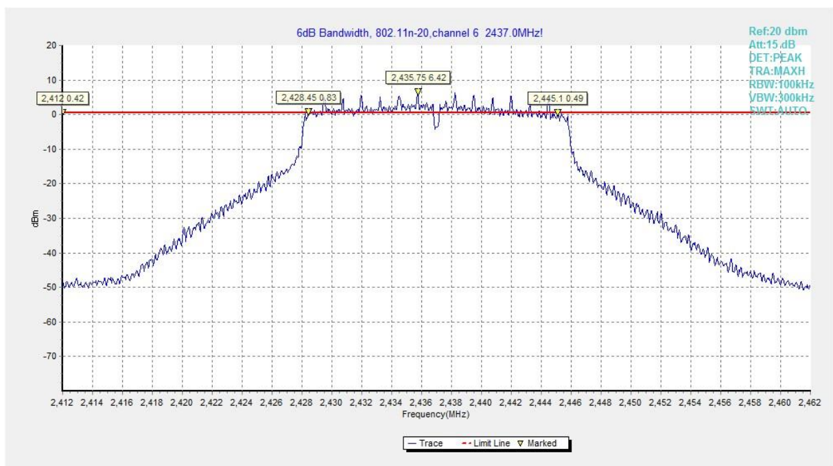
Fig.B.4.8 Occupied 6dB Bandwidth (802.11n-HT20, Ch 6)
