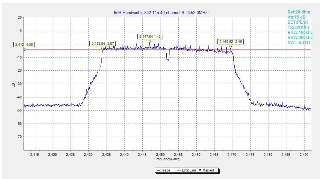
Fig.B.4.12 Occupied 6dB Bandwidth (802.11n-HT40, Ch 9)
