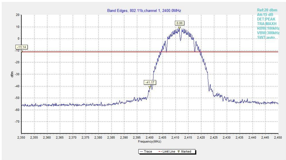
Fig.B.5.1 Band Edges (802.11b, Ch 1)
