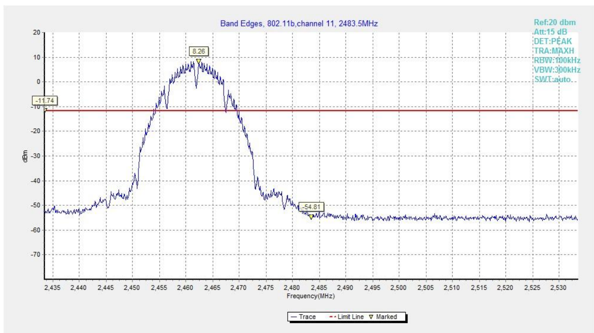
Fig.B.5.2 Band Edges (802.11b, Ch 11)
