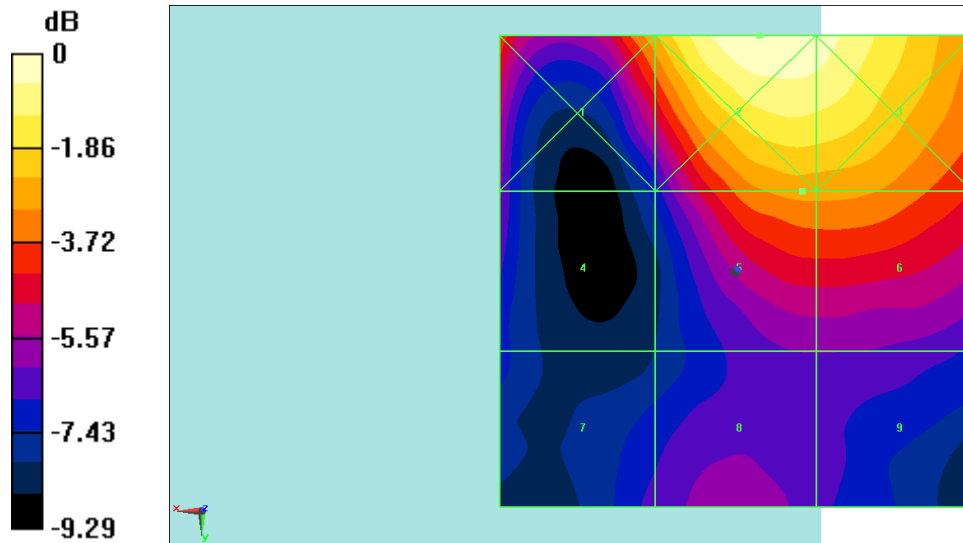
Fig B.7 HAC RF E-Field LTE Band41 Power Class 3 QPSK CH41490
