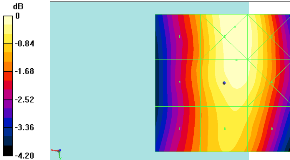
Fig B.1 HAC RF E-Field GSM 850 Low
