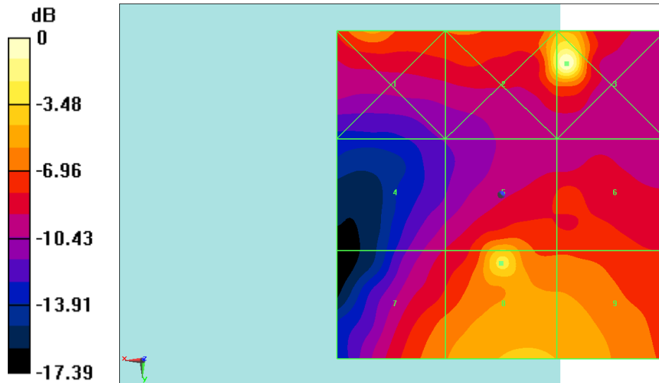
Fig B.4 HAC RF E-Field CDMA BC1 Low
