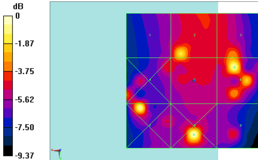
Fig B.5 HAC RF E-Field CDMA BC10 Low
