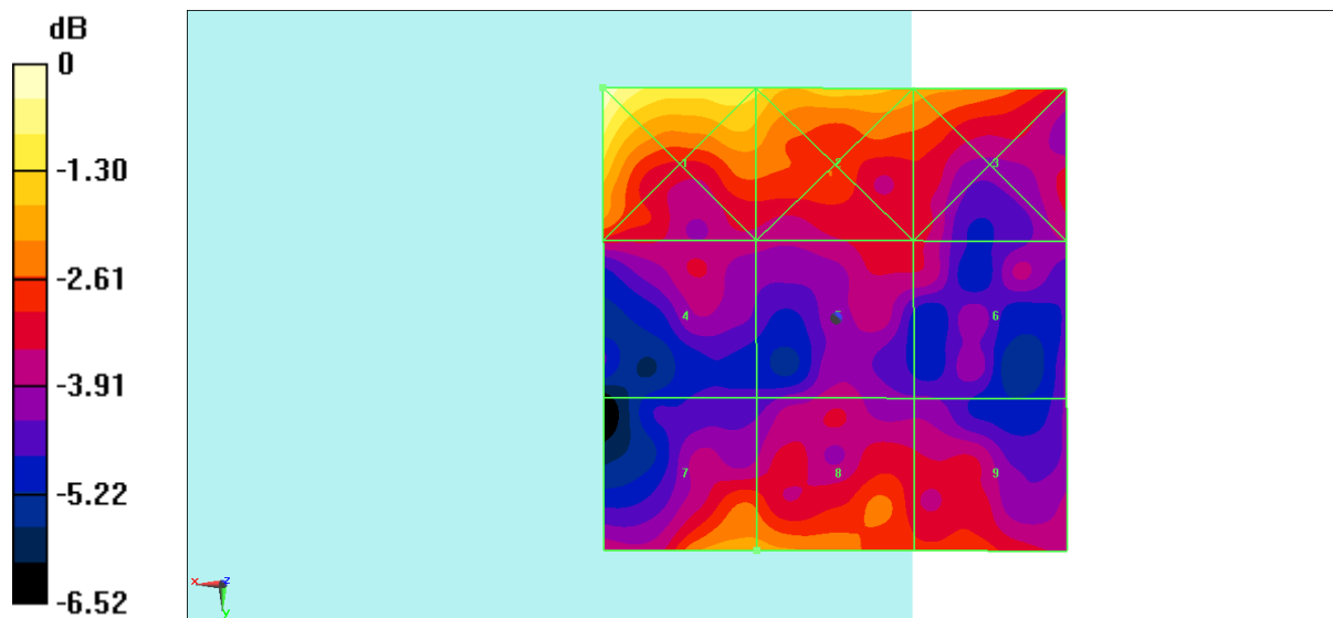
Fig B.2 HAC RF E-Field GSM 1900 Middle
