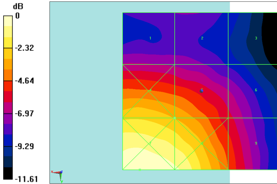
Fig B.8 HAC RF E-Field WiFi2.4G 11b
