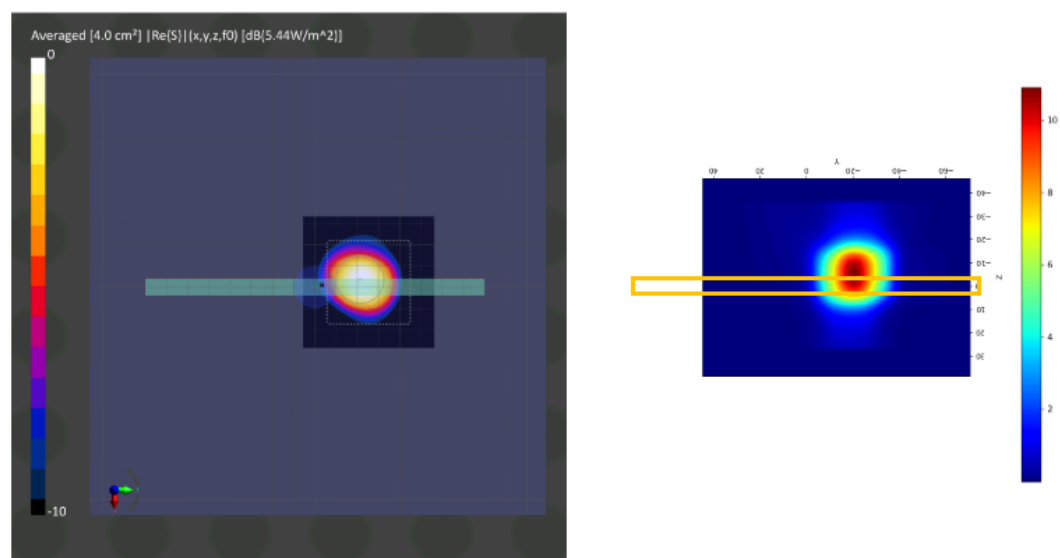
(a) Measurement (b) Simulation Module 2: Mid Channel, 4cm2 averaged power density
