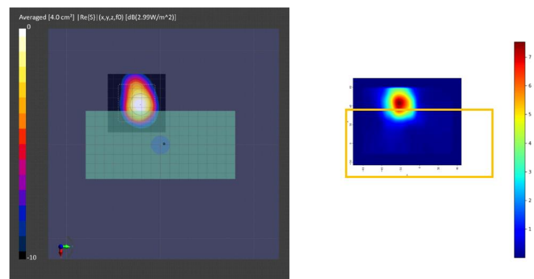
(b) Measurement (b) Simulation Module 2: Mid Channel, 4cm2 averaged power density
