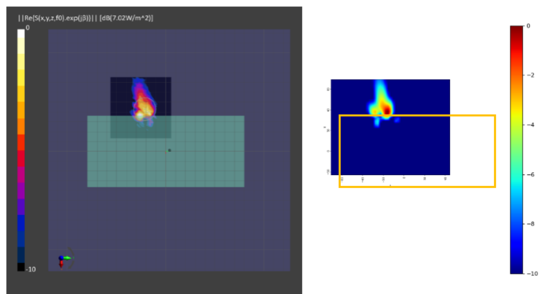
(a) Measurement (b) Simulation Module 2: Mid Channel, power density
