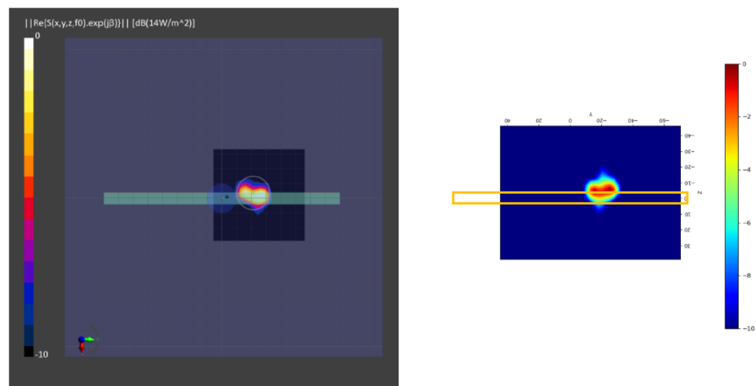
(a) Measurement (b) Simulation Module 2: Mid Channel, power density
