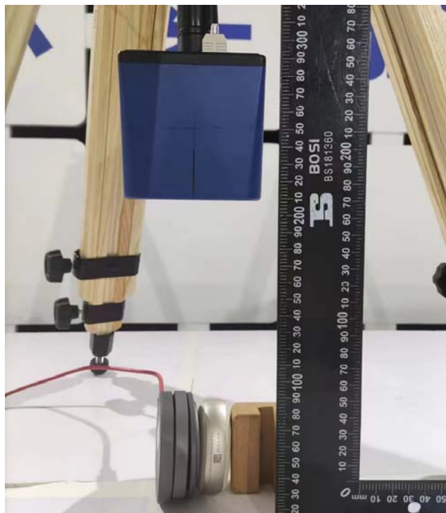
Right Side (Test distance: 15cm)
