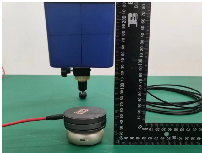
Back Side (Test distance: 15cm)
