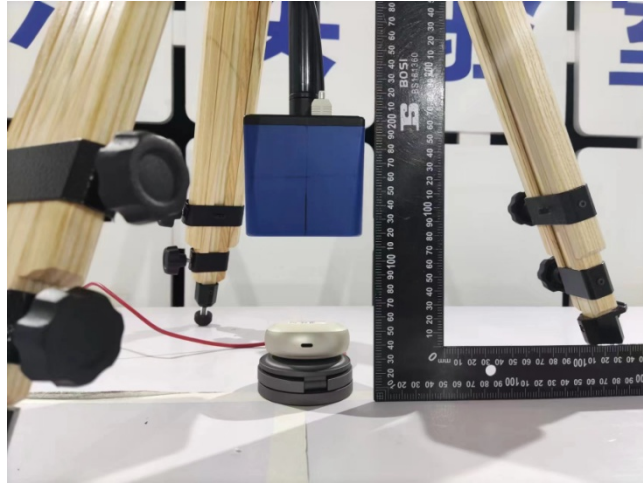
Front Side (Test distance: 15cm)
