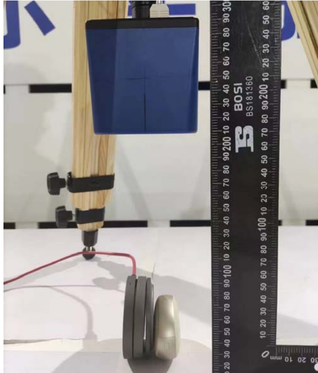
Top Side (Test distance: 15cm)
