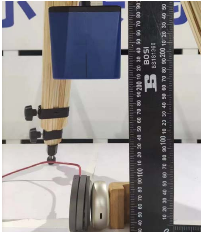
Left Side (Test distance: 15cm)
