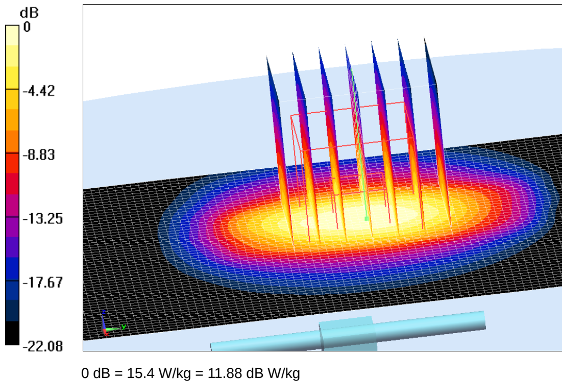
Fig.B.1. Validation 2450MHz 250mW
