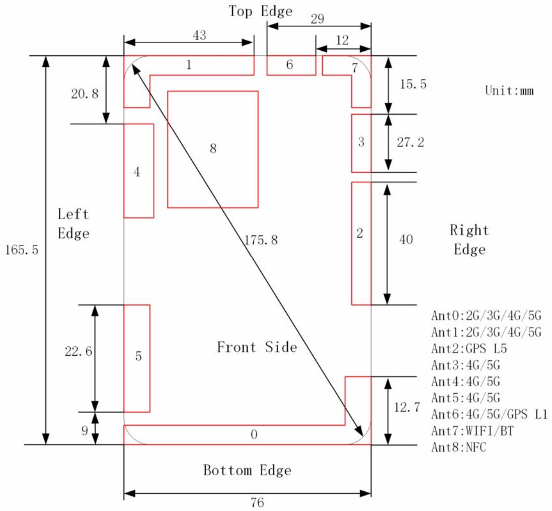
Fig 5 Antenna location&dimension
