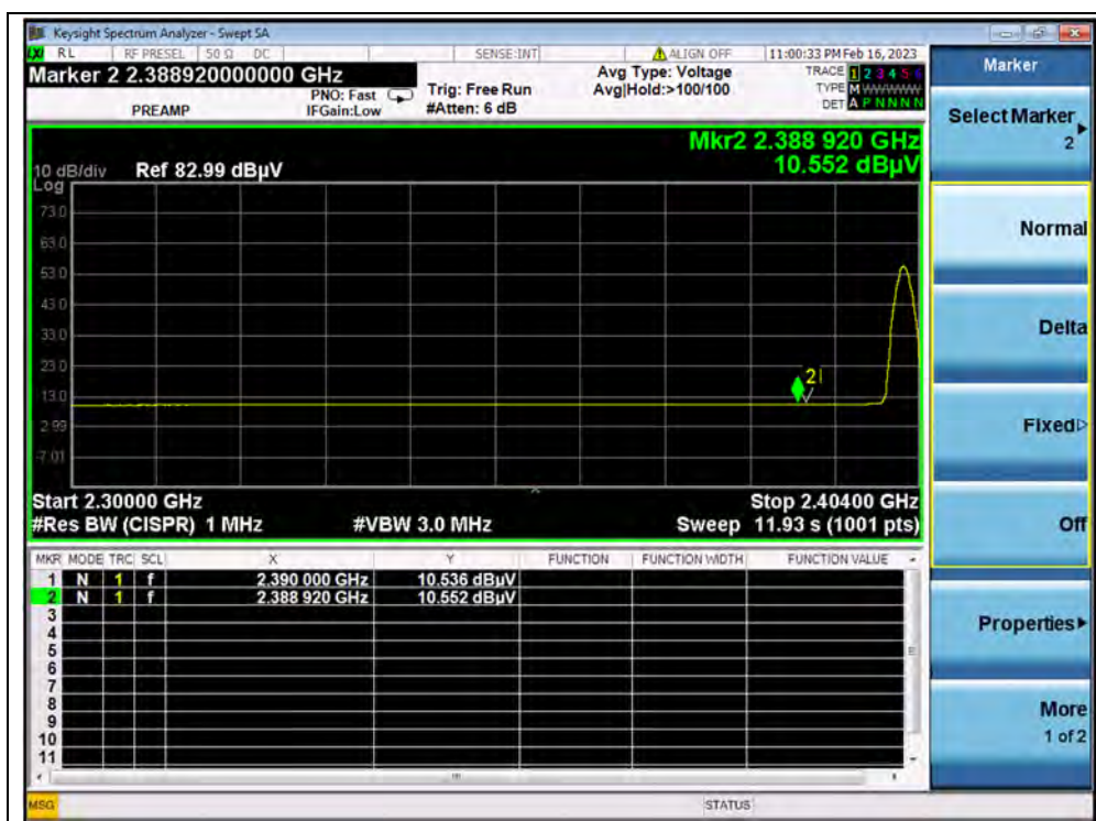
(AVERAGE, Channel 0)
