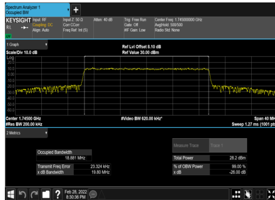
B2_N66(20M)_CP-OFDM_16 QAM_Outer_Full_Mid_CH
