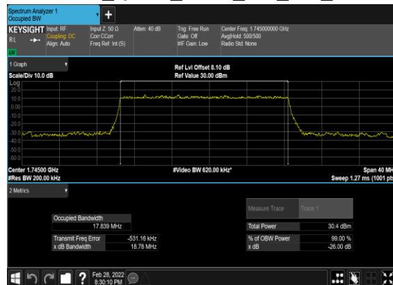
B2_N66(20M)_DFT-s- OFDM_QPSK_Outer_Full_Mid_CH
