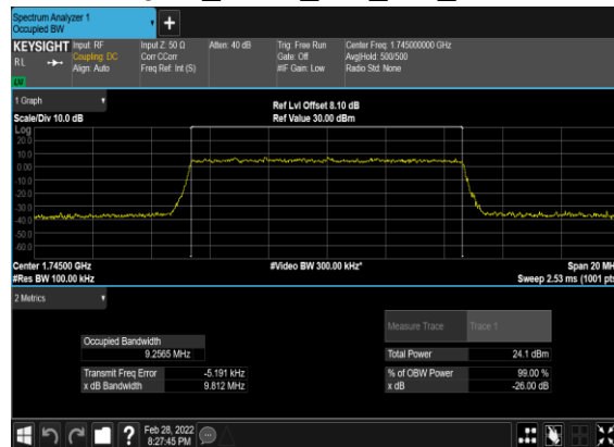
B2_N66(10M)_CP-OFDM_256 QAM_Outer_Full_Mid_CH
