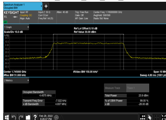
B2_N66(5M)_CP-OFDM_256 QAM_Outer_Full_Mid_CH
