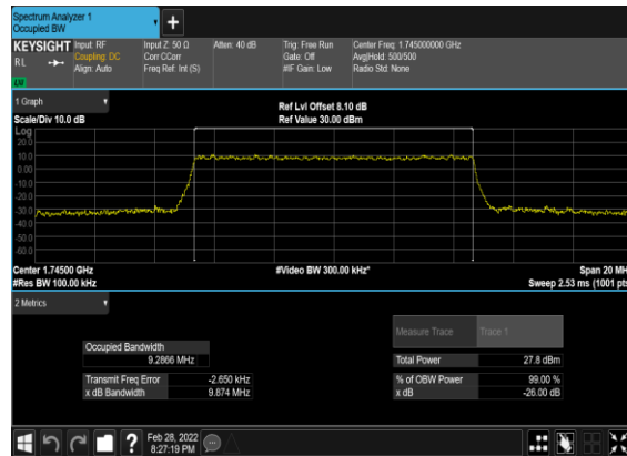
B2_N66(10M)_CP-OFDM_16 QAM_Outer_Full_Mid_CH
