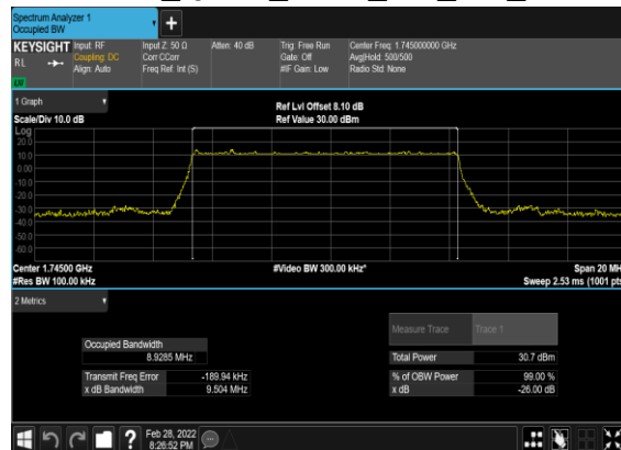
B2_N66(10M)_DFT-s- OFDM_QPSK_Outer_Full_Mid_CH
