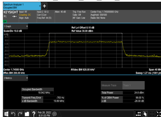
B2_N66(20M)_CP-OFDM_256 QAM_Outer_Full_Mid_CH
