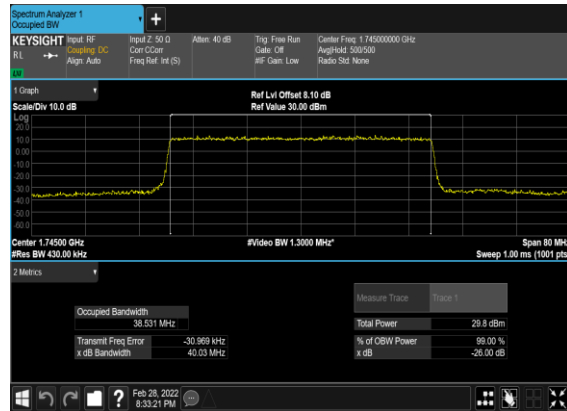
B2_N66(40M)_DFT-s- OFDM_QPSK_Outer_Full_Mid_CH
