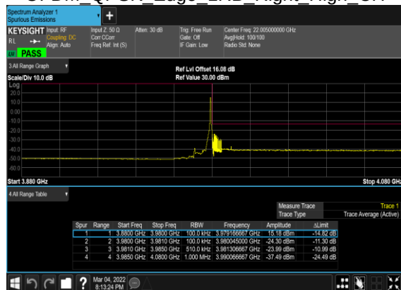
N77(10M)_DFT-s- OFDM QPSK Edge 1RB Right High CH
