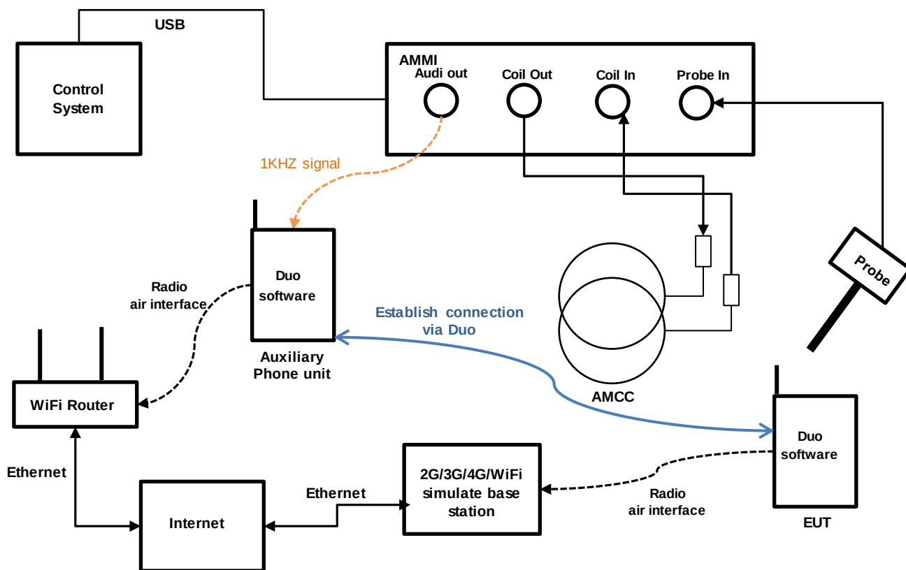
Test Setup for 3rd party VoIP calling
