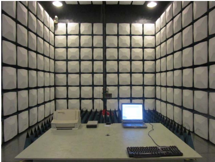
Radiated Emissions –Front View (Above 1GHz) For USB
