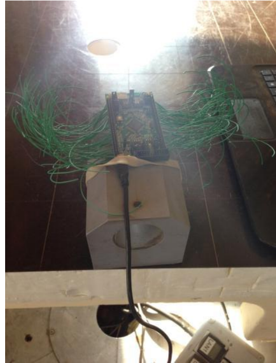
Test setup on OATS
