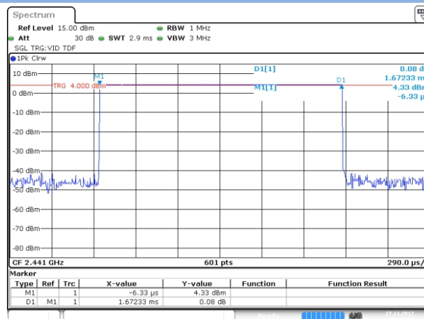
GFSK DH3
