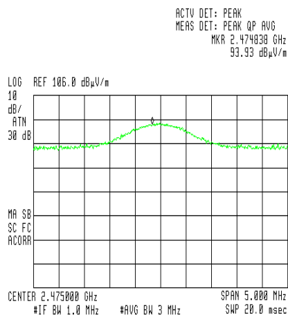
Figure 16. Field Strength of Fundamental. Antenna Polarization: HORIZONTAL Channel: High
