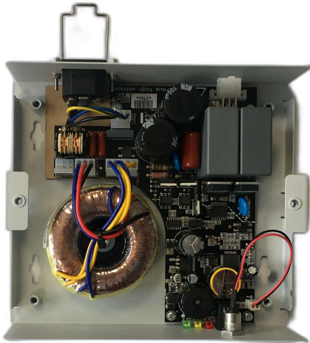
Callidus AM deactivator, TOP board
