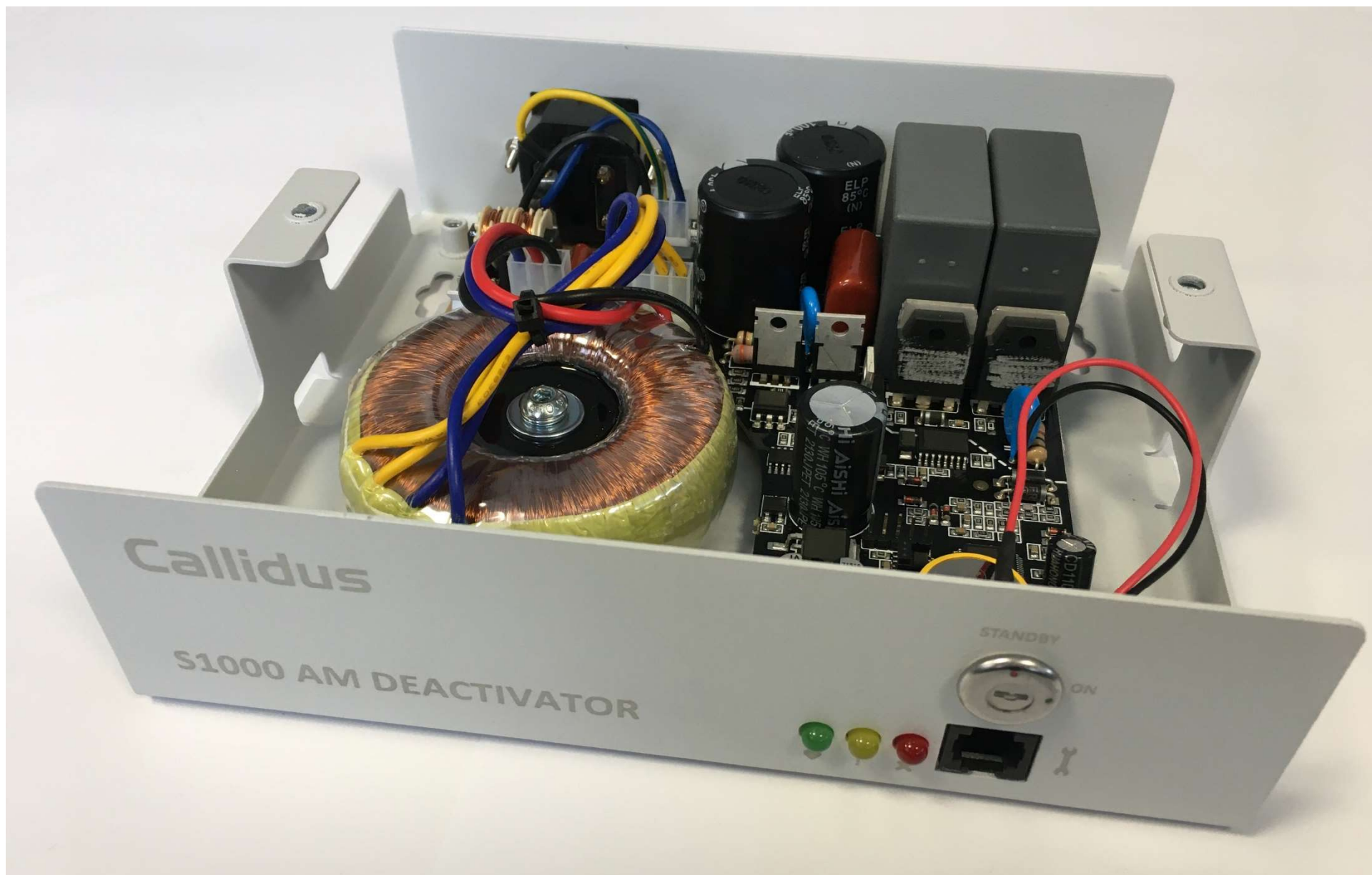
Callidus AM deactivator, without cover
