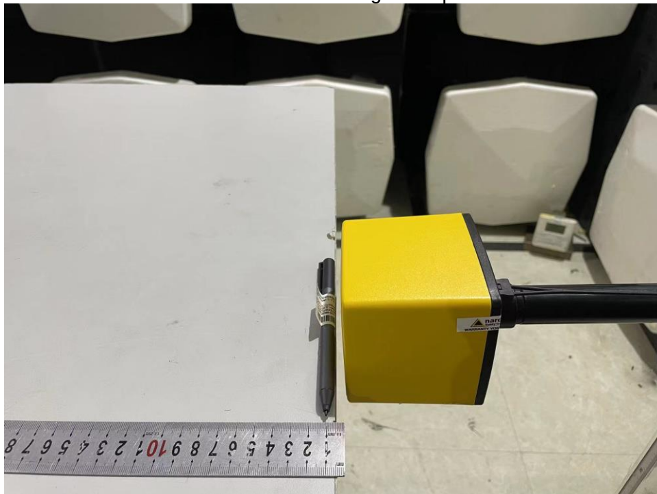
H-Field & E-Field Strength test photos
