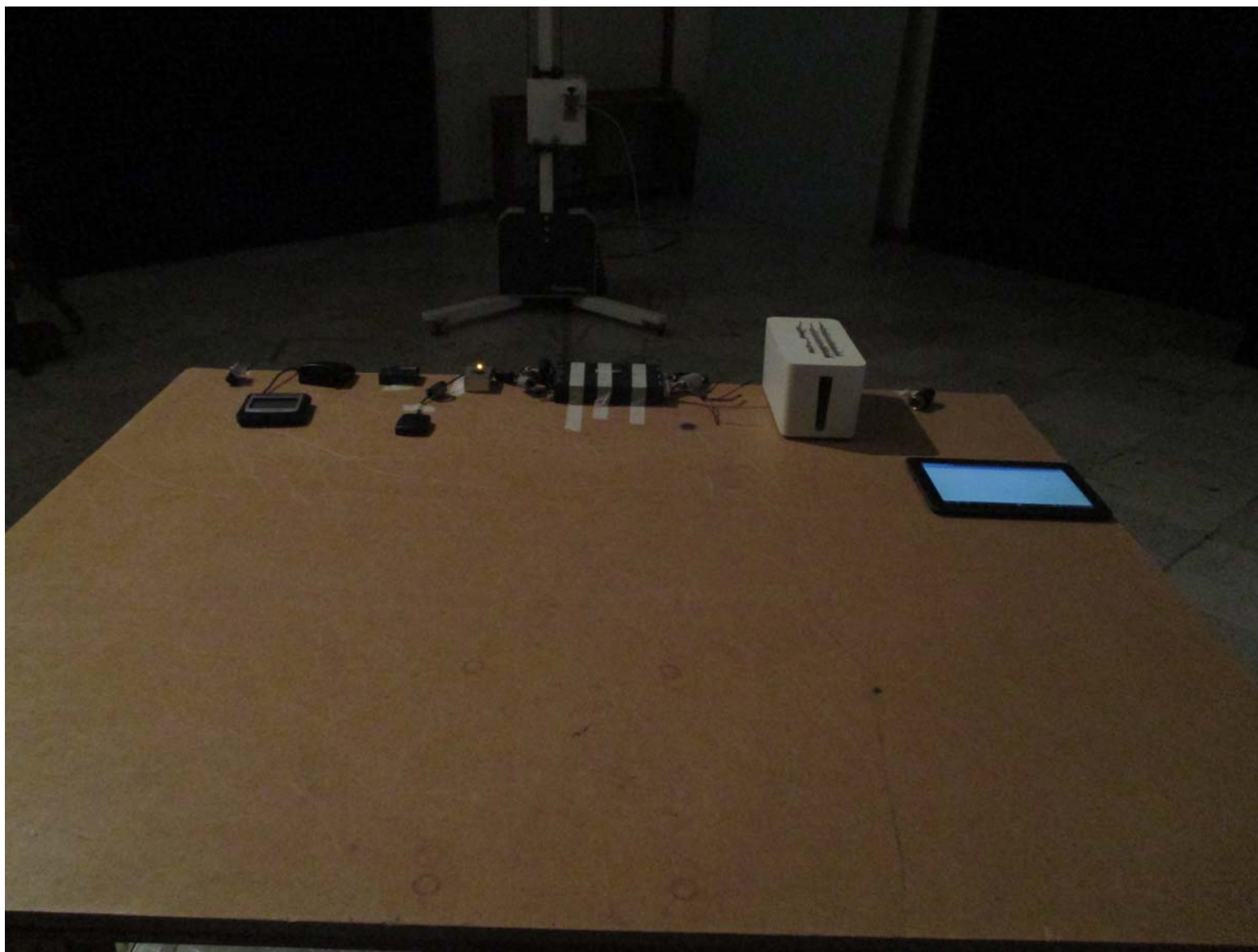
[ERTS-5000] 18 GHz to 26.5 GHz Radiated Emission Front Side
