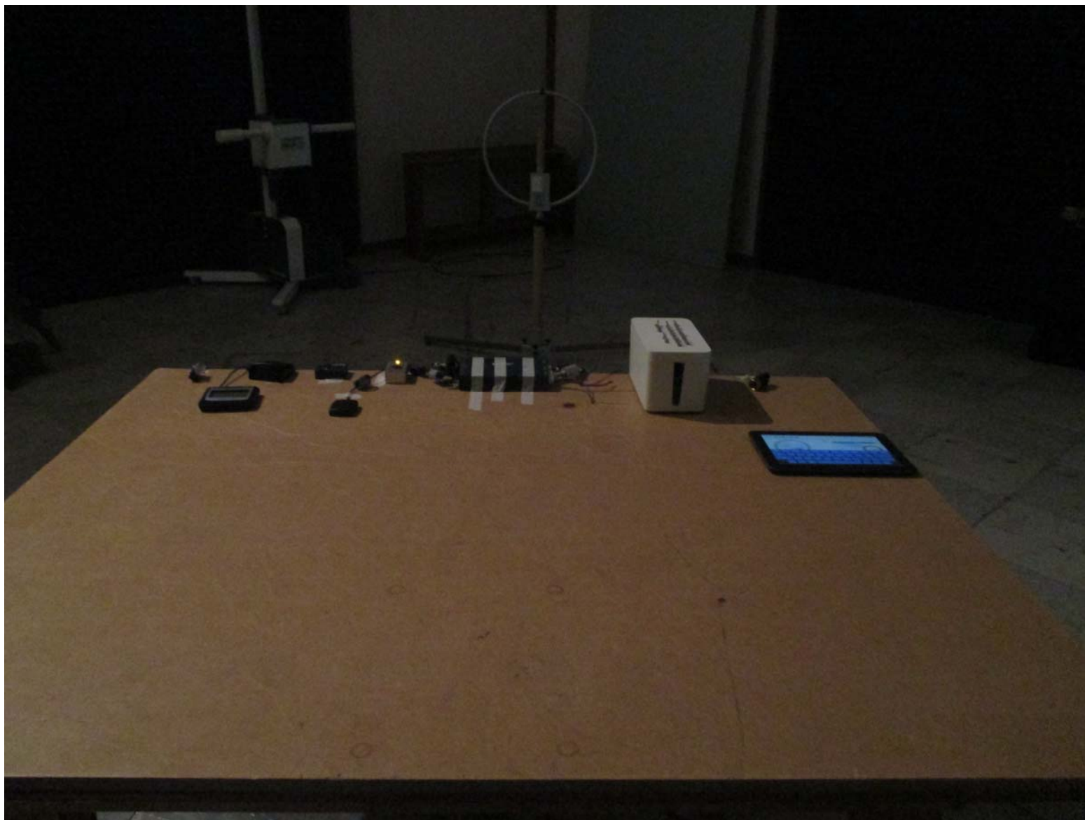
[ERTS-5000] 9 kHz to 30 MHz Radiated Emission Front Side
