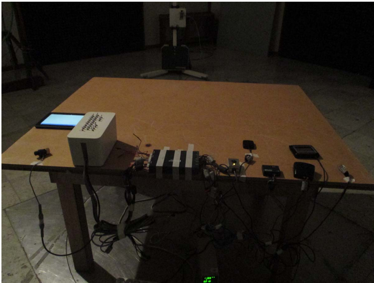
[ERTS-5000] 18 GHz to 26.5 GHz Radiated Emission Rear Side
