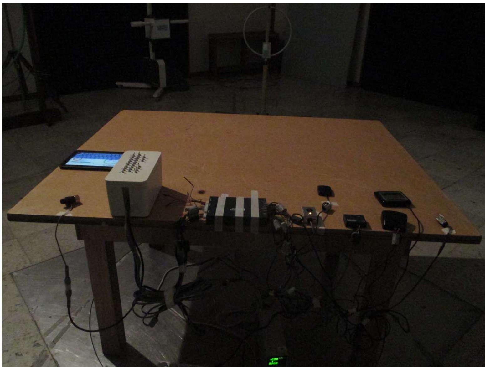
[ERTS-5000] 9 kHz to 30 MHz Radiated Emission Rear Side
