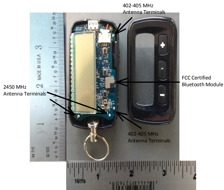
BPOP Assembly Photo:
