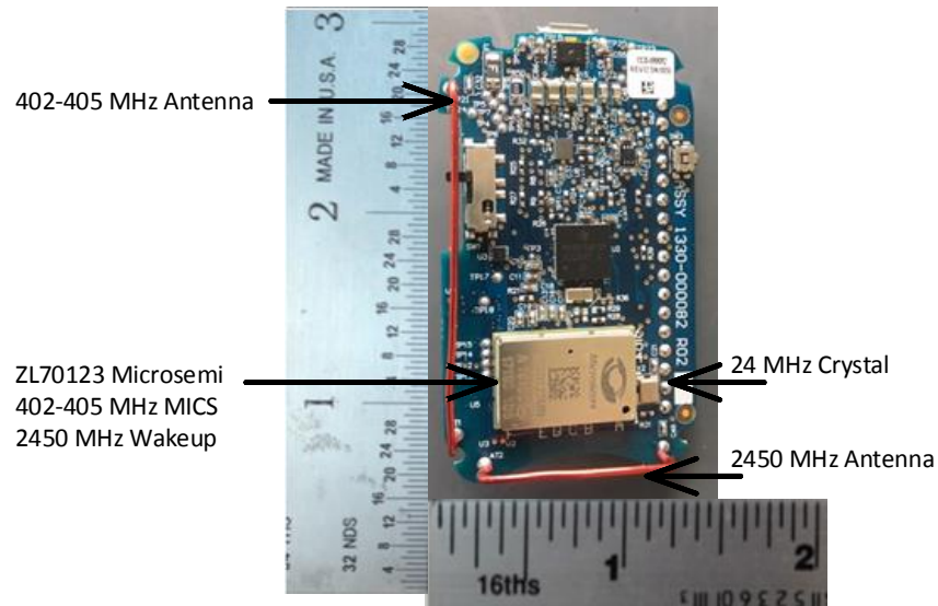
BPOP Assembly Photo:
