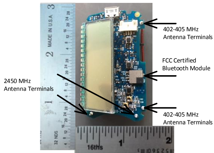
Circuit Board Photo (Front Display Side):
