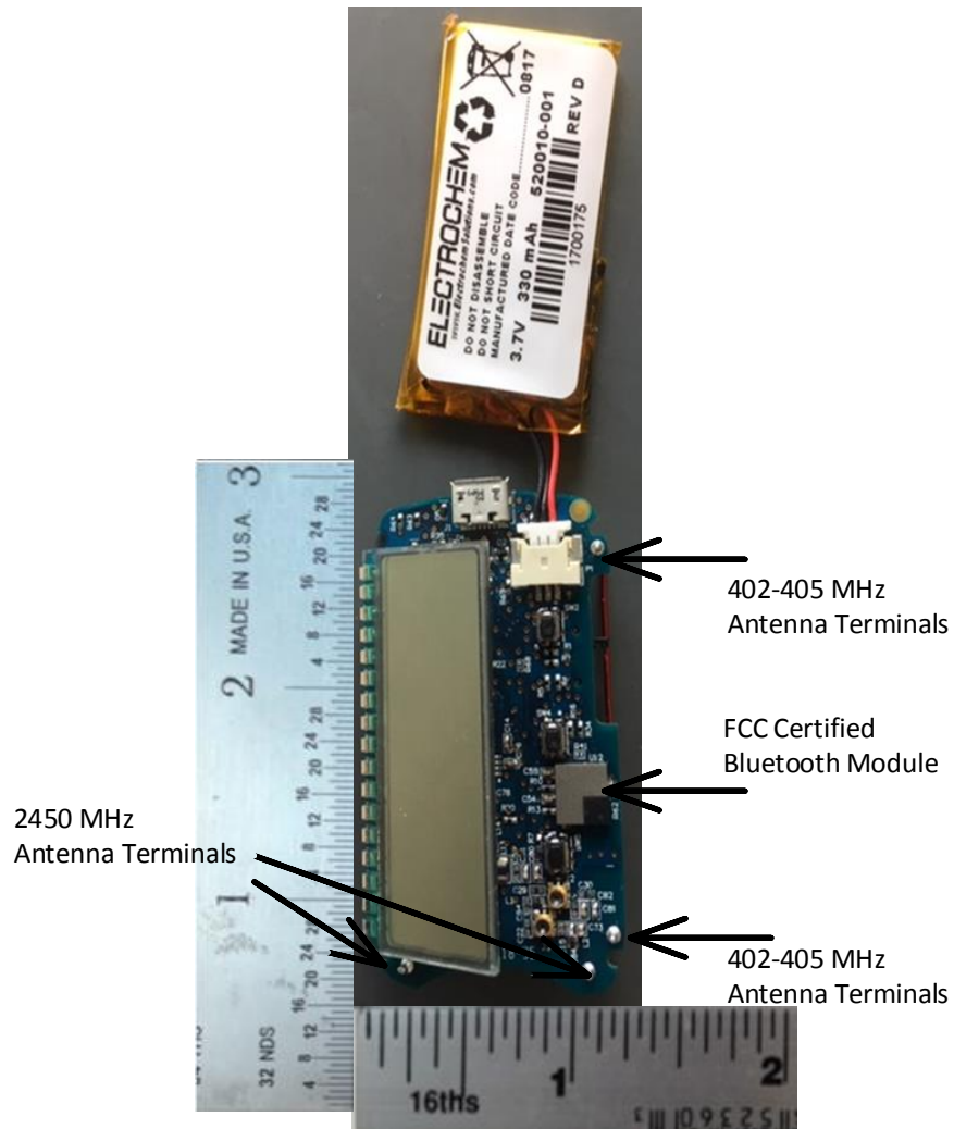
Circuit Board Photo (Front Display Side With Battery):
