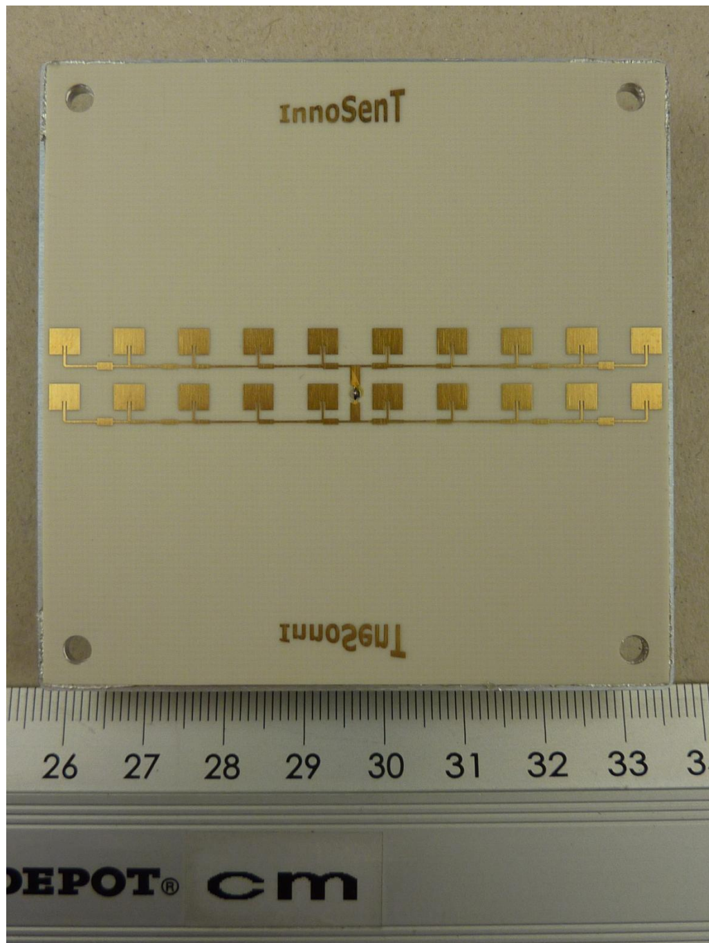
132431_m.JPG: CRA61, Antenna PCB, top view
