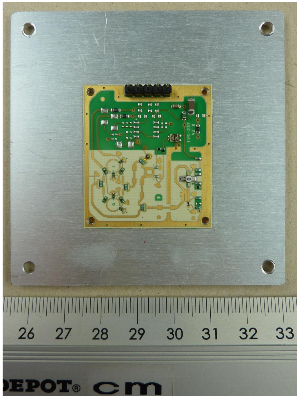
132431_n.JPG: detail view to RF-module, cover removed
