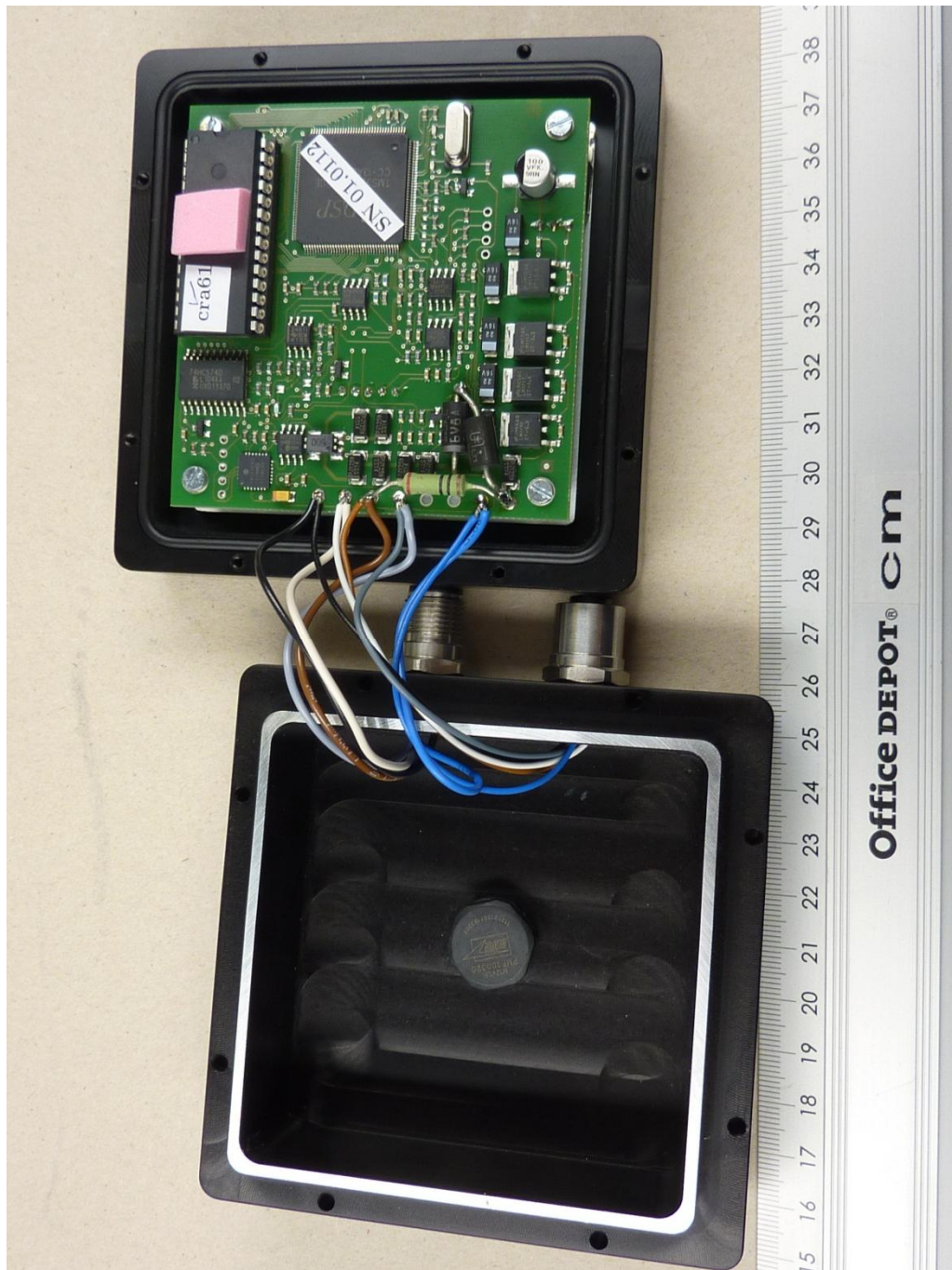
132431_k.JPG: CRA61, internal view 1
