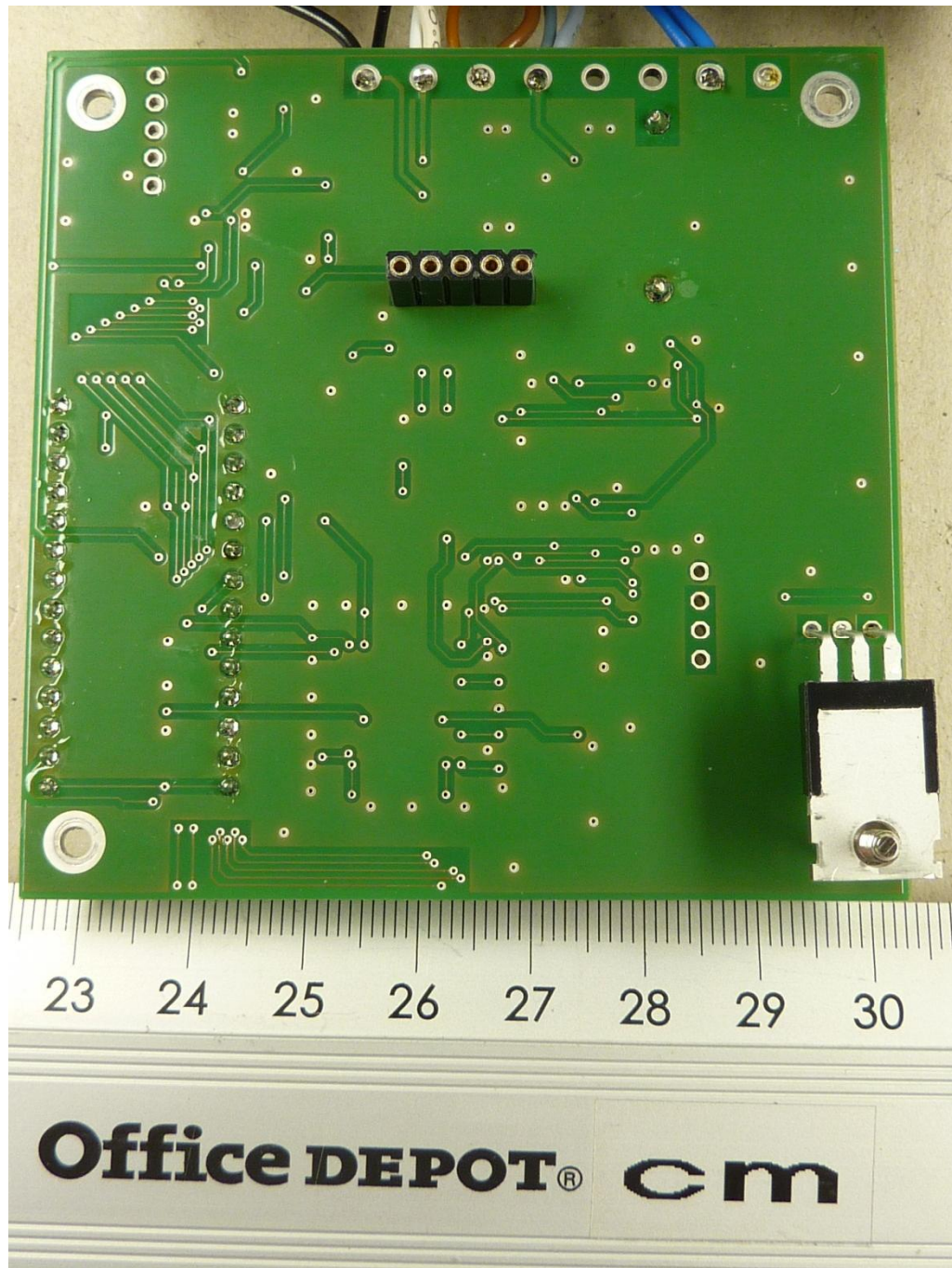
132431_r.JPG: CRA61, main PCB, bottom view
