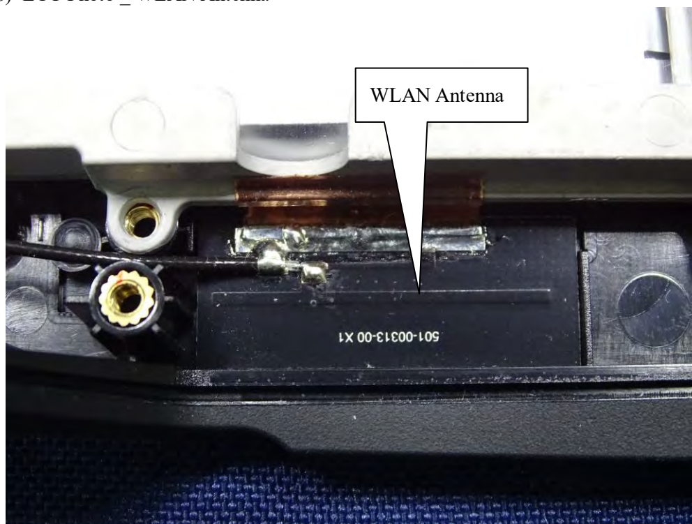
(78) EUT Photo _ WLAN Antenna
