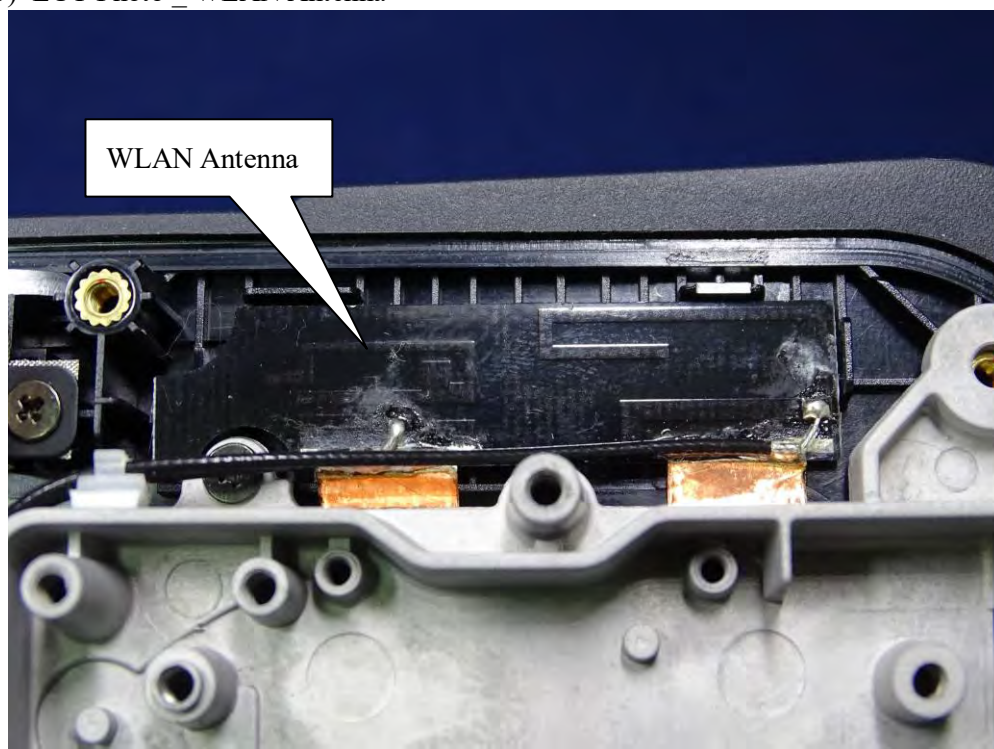
(75) EUT Photo _ WLAN Antenna
