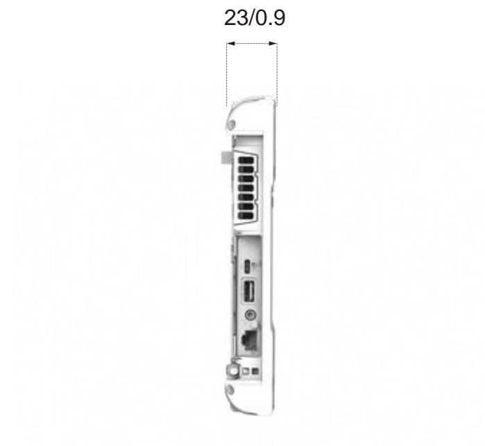
Figure 8. Side View Dimensions
