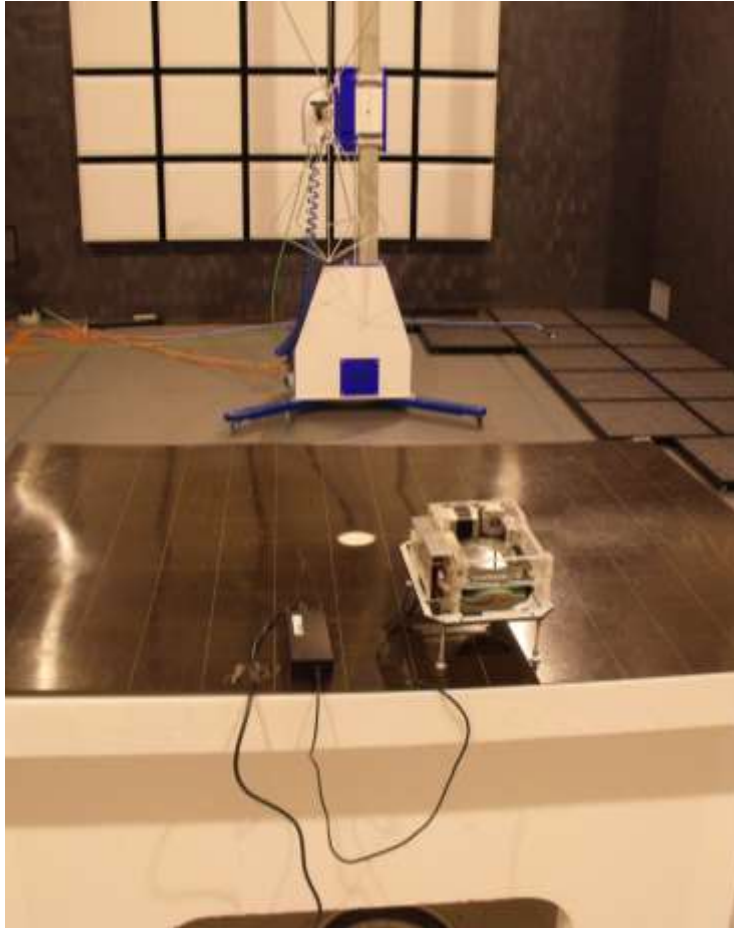
Figure 3: Radiated emission test from 30 MHz to 200 MHz in SAC
