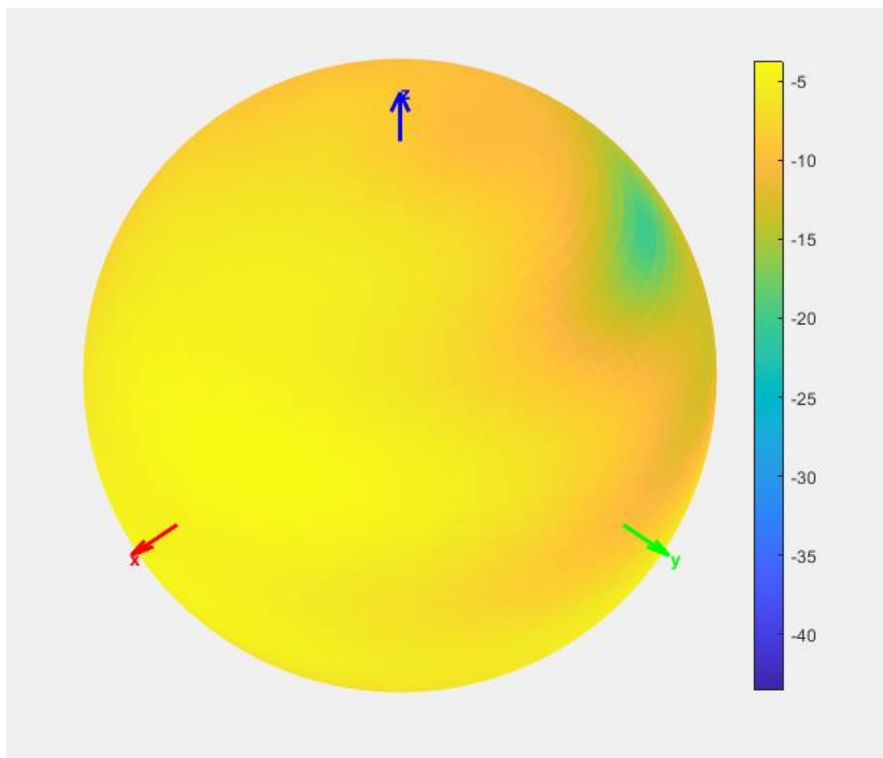
Figure 6-3: 3D gain pattern @921.4 MHz
