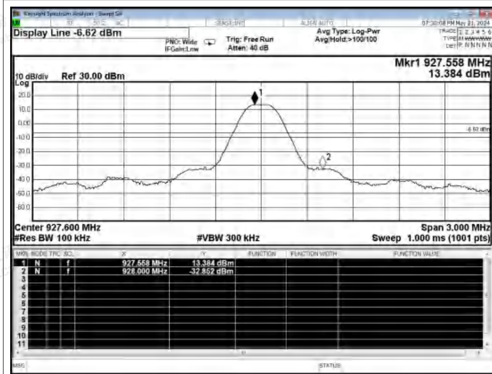
Band Edge NVNT 150Kbps 927.6MHz Ant1 No-Hopping Ref
