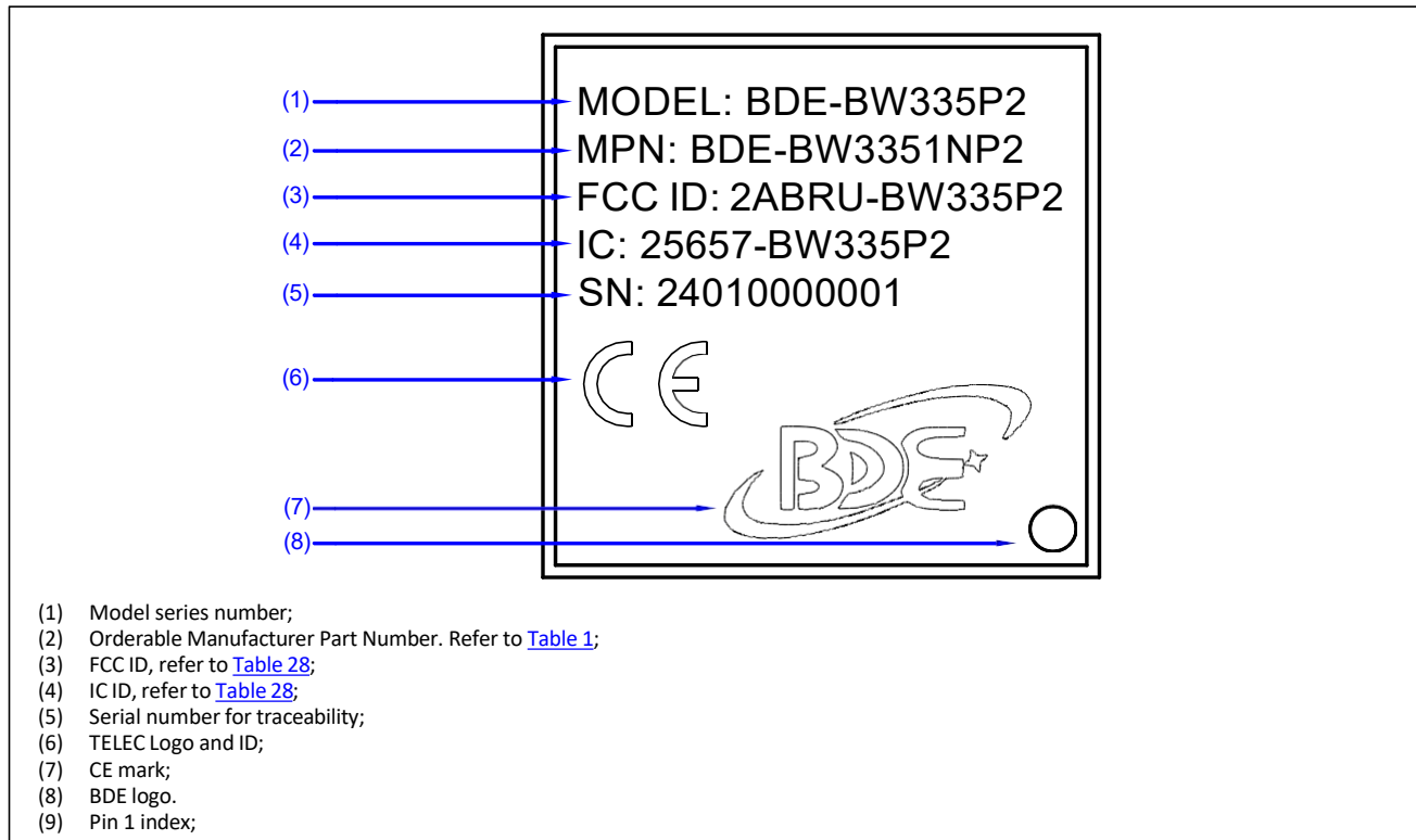
Figure 18. Module Marking
