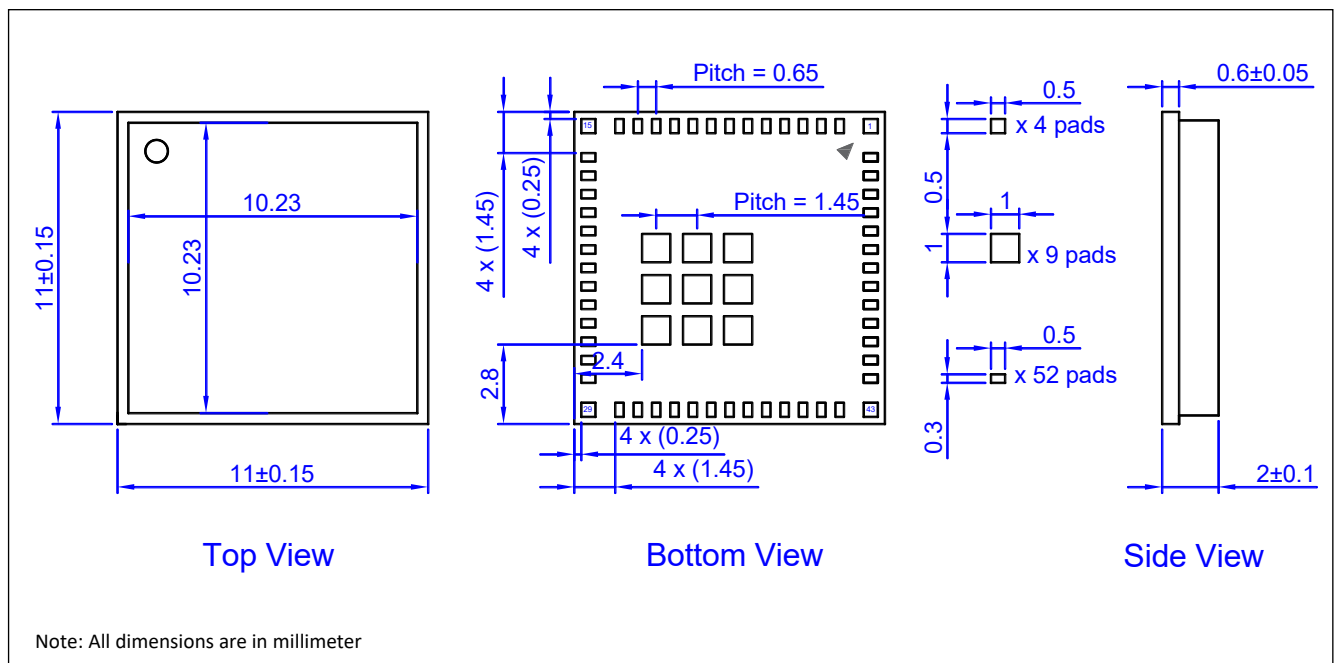
Figure 13. Mechanical Drawing of BDE-BW330XN1
