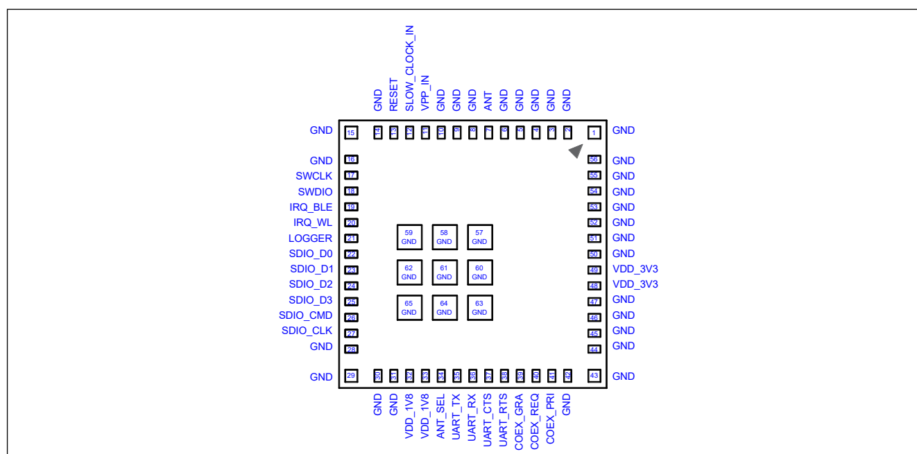
Figure 5. Pin Diagram of BDE-BW330XN1 (Bottom View)
