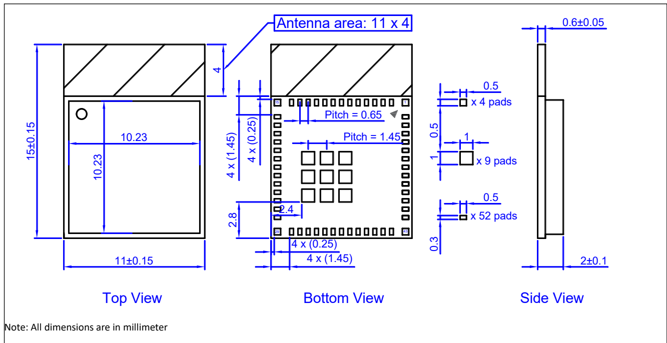
Figure 14. Mechanical Drawing of BDE-BW330XA1, BDE-BW330XU1
