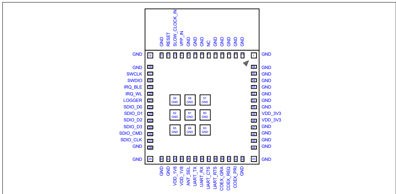
Figure 6. Pin Diagram of BDE-BW330XA1, BDE-BW330XU1 (Bottom View)
