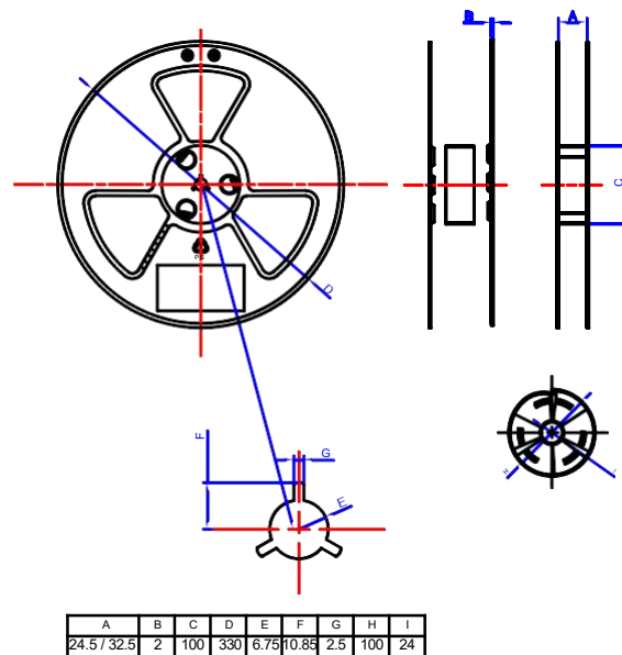
Figure 19. Carrier Tape Drawing for BDE-BW330XUPX variants
