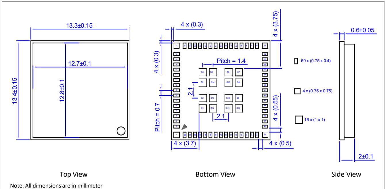
Figure 12. Mechanical Drawing of BDE-BW330XNP1 and BDE-BW330XNP2
