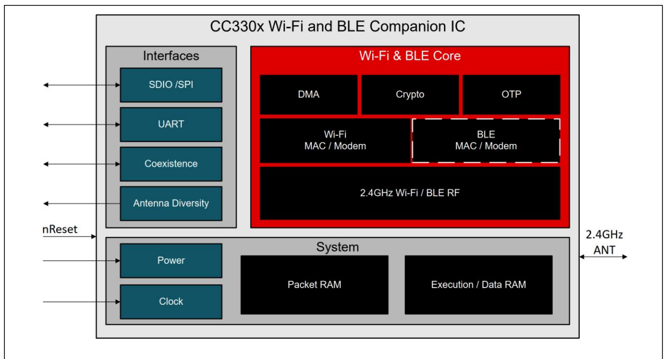
Figure 3. The block diagram of CC3301 (Adopted from CC3301 Datasheet)
