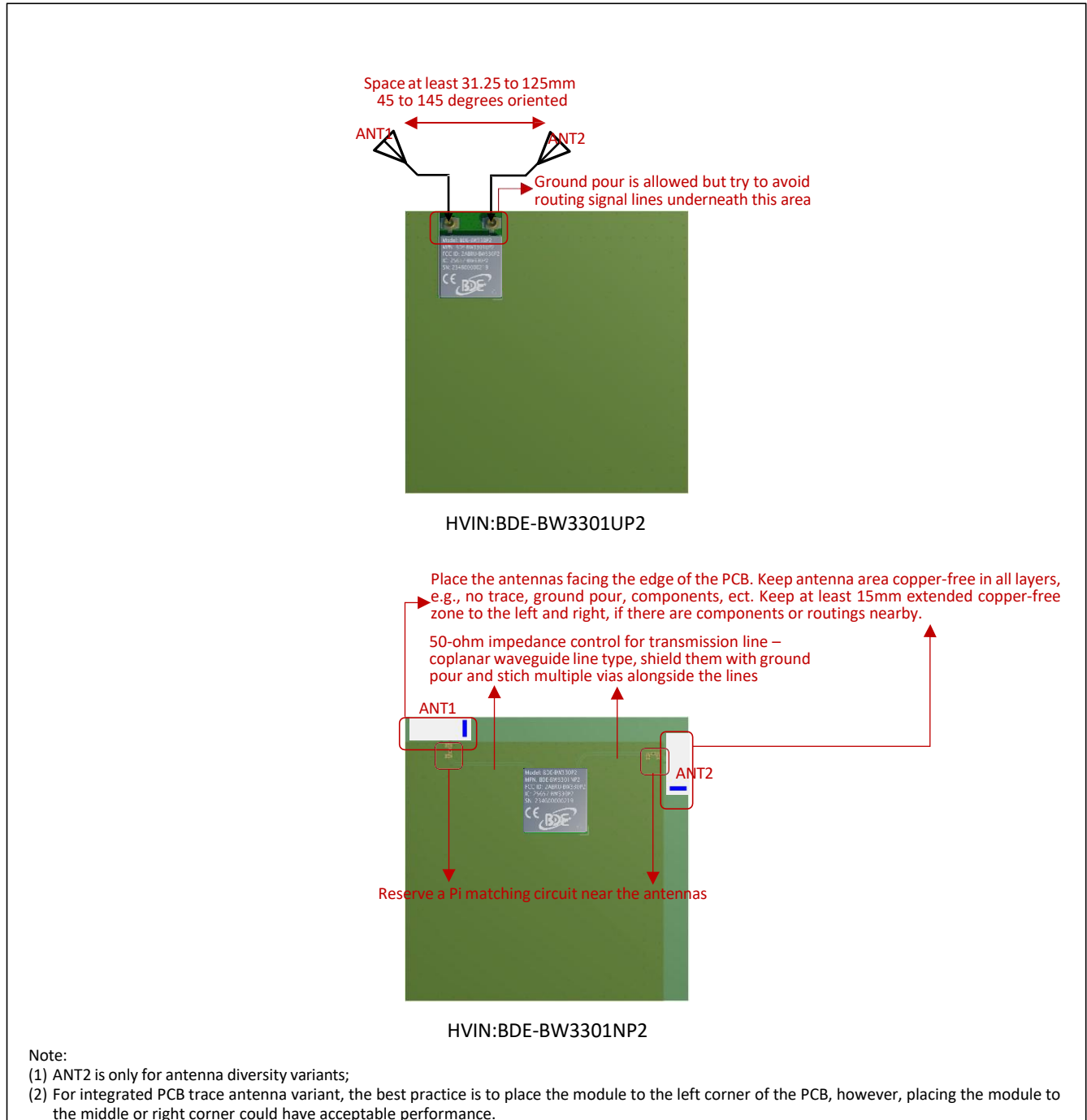
Figure 17. Recommended Module Placement
