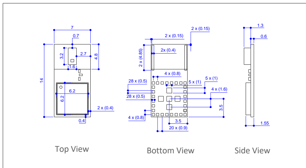
Figure 4-1. Mechanical Drawing
