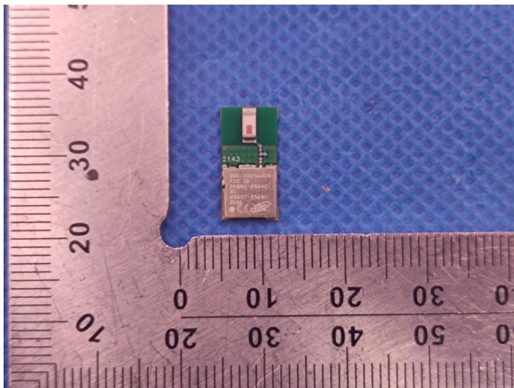
Model: BDE-BD2564CA TOP VIEW OF EUT
