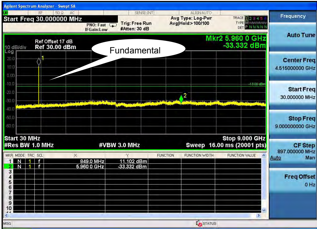
Test Mode:GPRS 850 - High Channel
