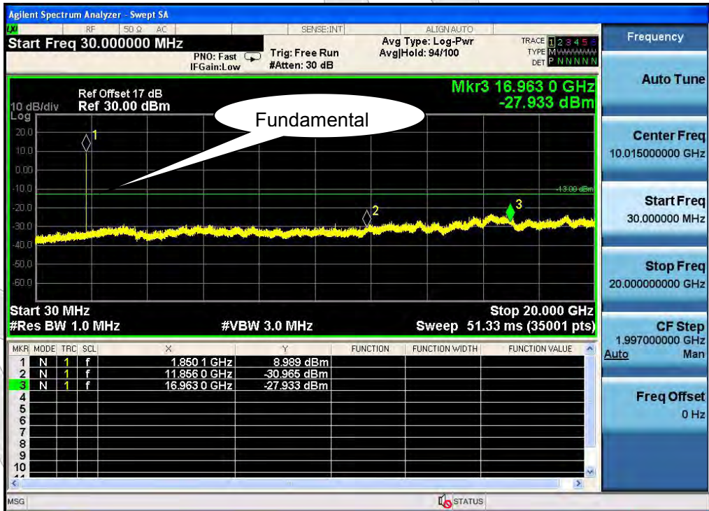
Test Mode:PCS1900 - Low Channel
