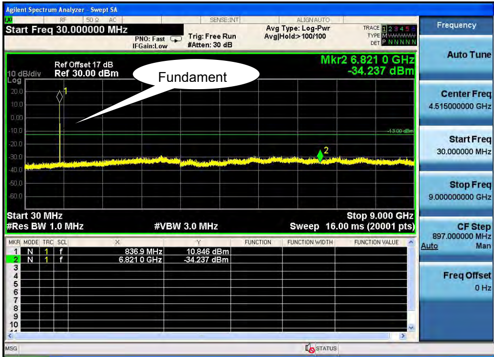
Test Mode:GSM 850 Middle Channel
