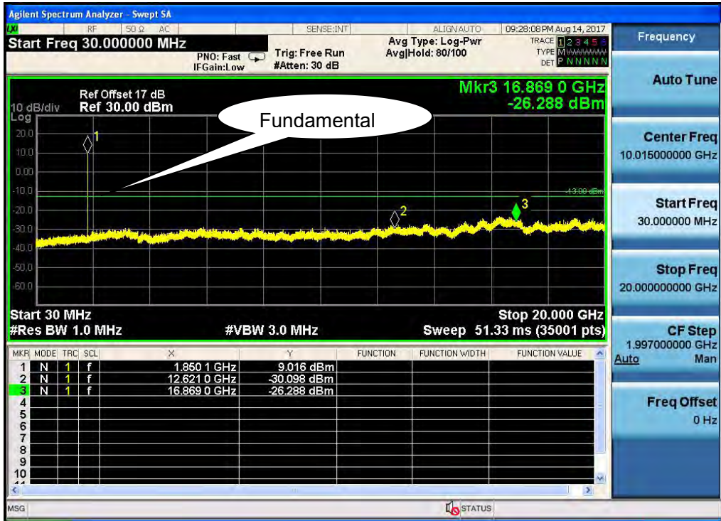
Test Mode:GPRS 1900 - Low Channel
