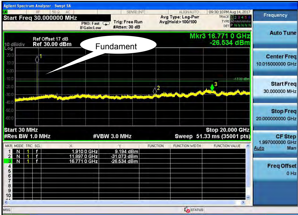
Test Mode:GPRS 1900 - High Channel
