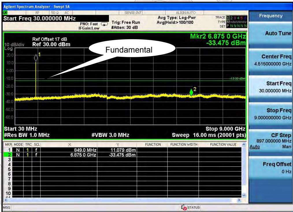
Test Mode:GSM 850 - High Channel
