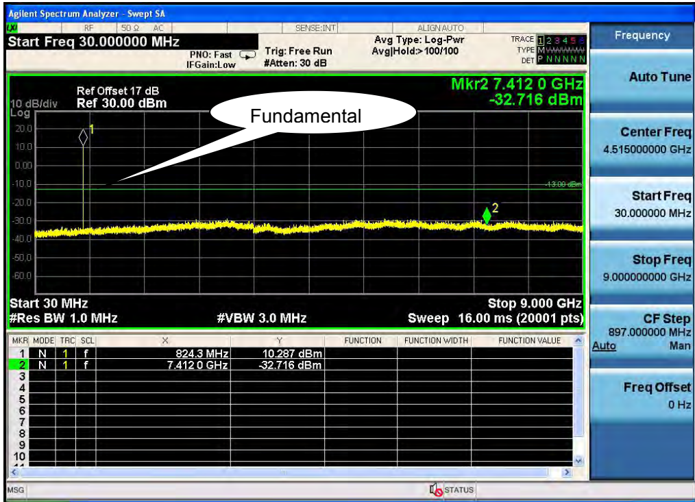
Test Mode:GPRS 850 - Low Channel
