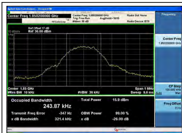
PCS 1900 BW - Low CH 1850.2MHz
