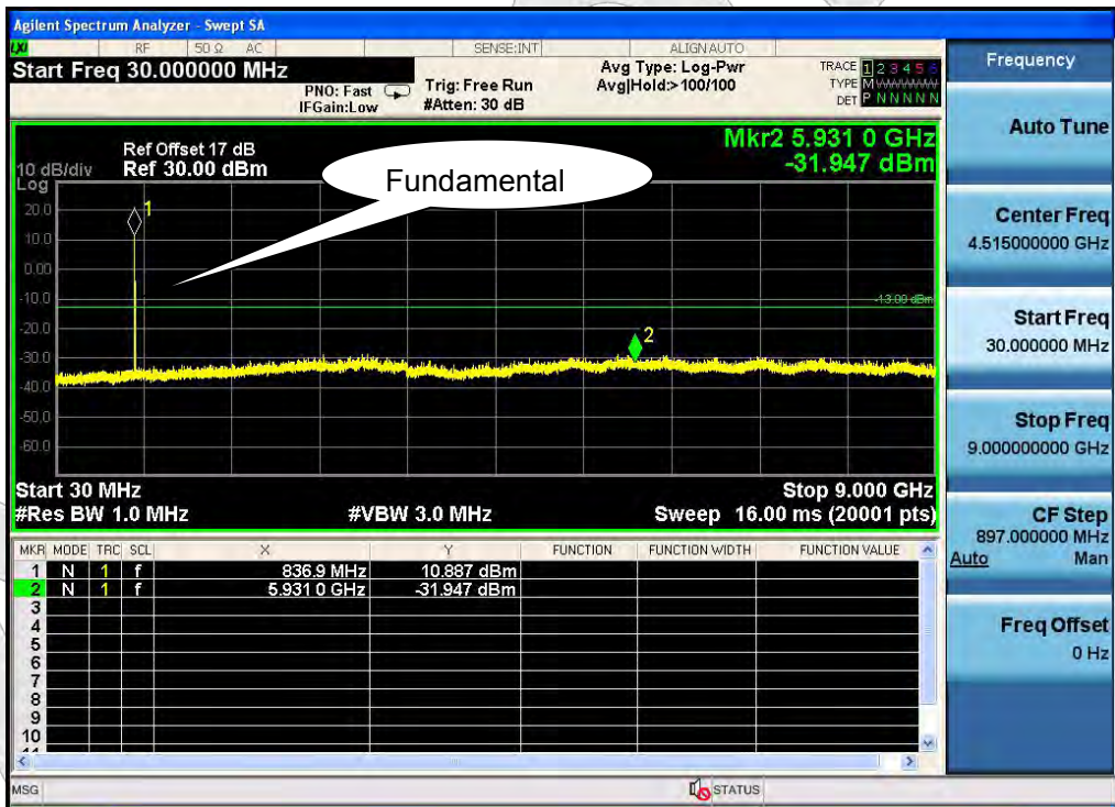
Test Mode:GPRS 850 - Middle Channel
