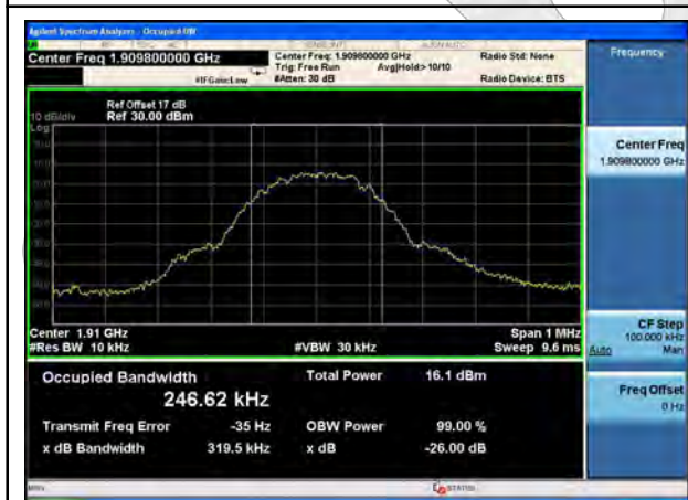
PCS 1900 BW - High CH 1909.8MHz
