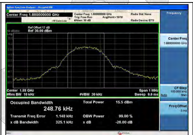
PCS 1900 BW - Mid CH 1880MHz
