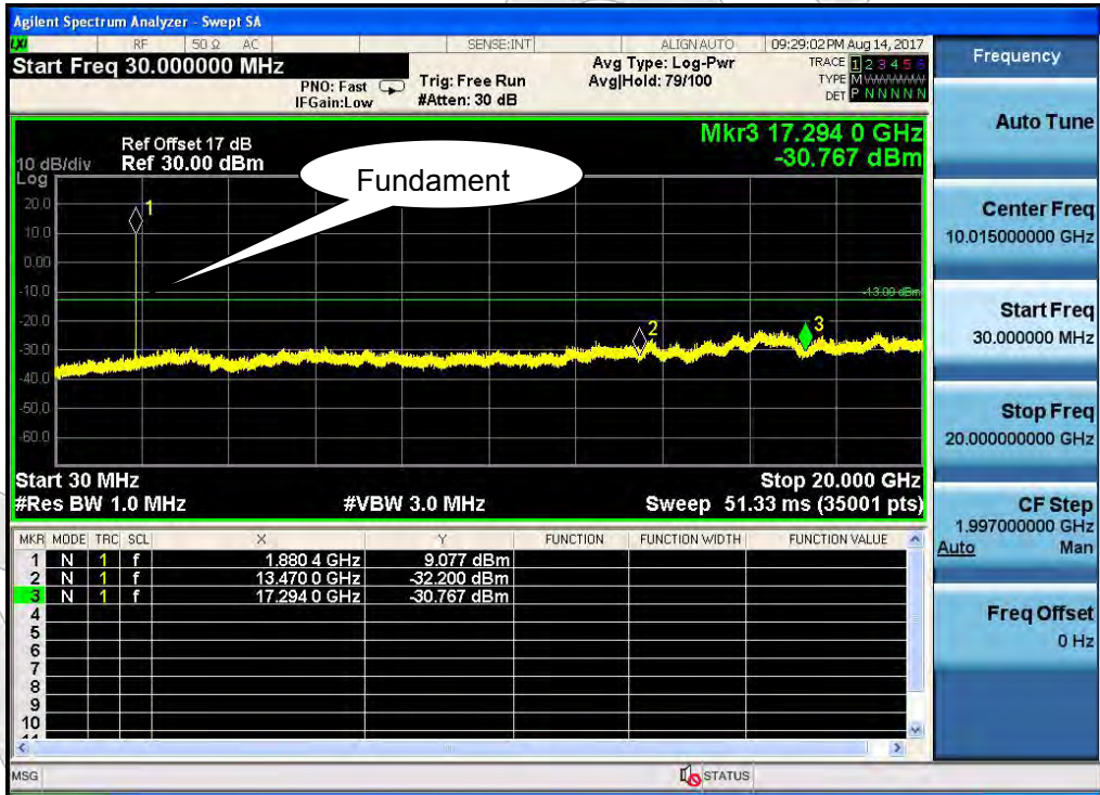
Test Mode:GPRS 1900 - Middle Channel
