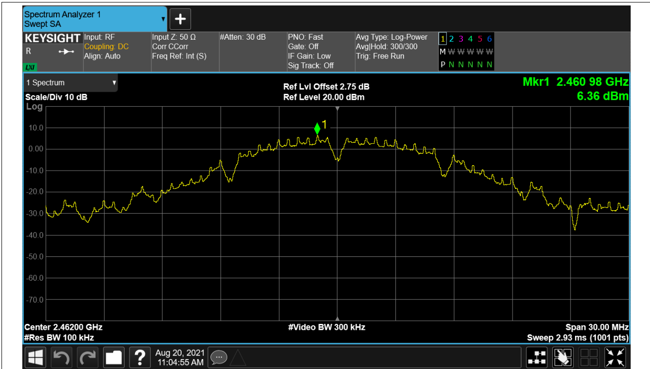
Tx. Spurious NVNT b 2462MHz Ant1 Emission
