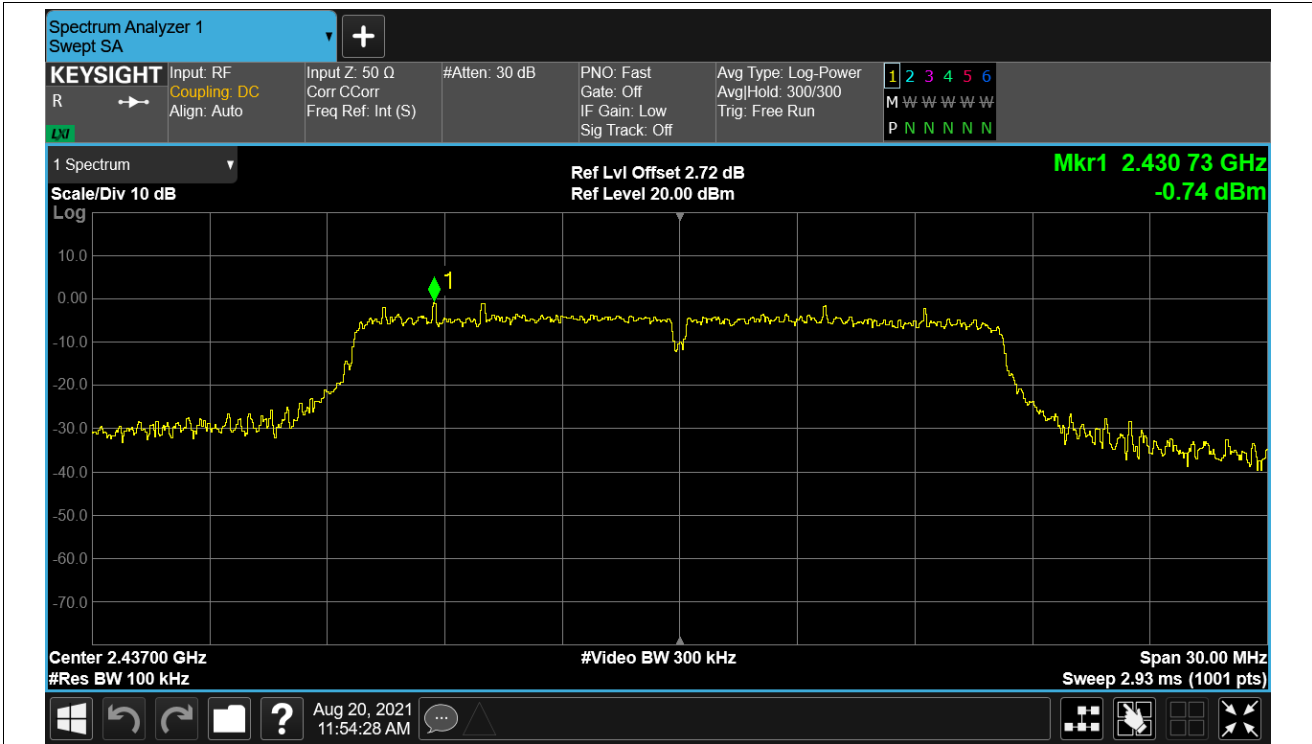
Tx. Spurious NVNT g 2437MHz Ant1 Emission
