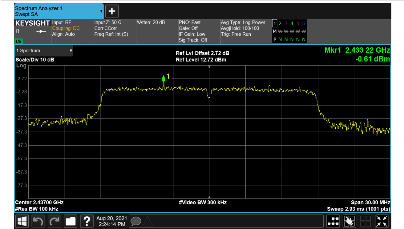
Tx. Spurious NVNT n20 2437MHz Ant1 Emission
