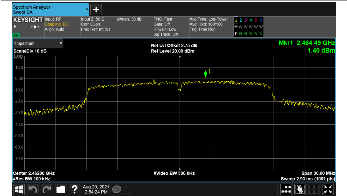
Tx. Spurious NVNT n20 2462MHz Ant1 Emission
