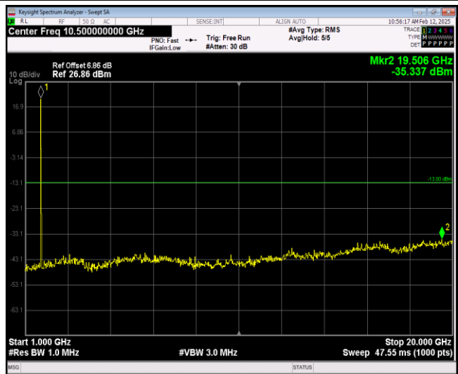
Band4-20MHz-64QAM-20175-1RB#0-Range2:1000~20000MHz
