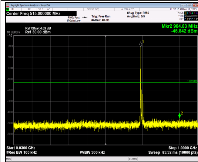
Band12-10MHz-64QAM-23095-1RB#0-Range1:30~-1000MHz
