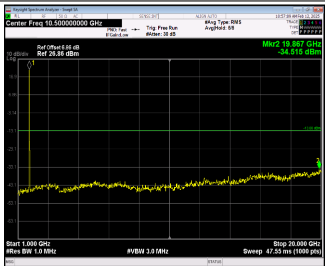
Band4-20MHz-64QAM-20300-1RB#0-Range2:1000~20000MHz
