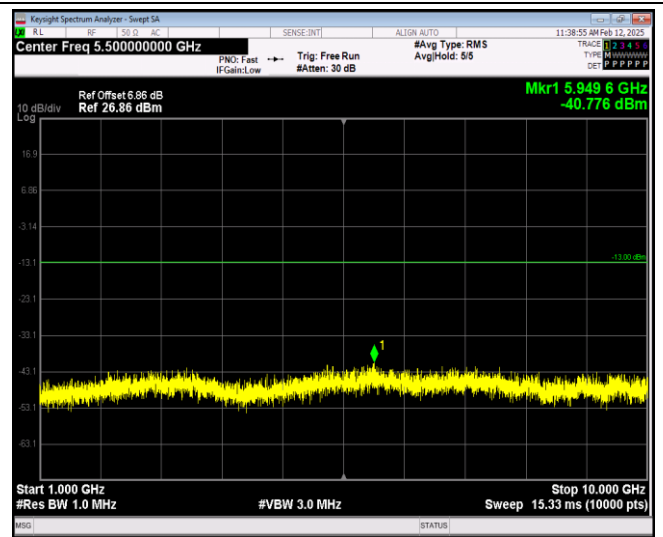
Band12-10MHz-64QAM-23060-1RB#0-Range2:1000~10000MHz
