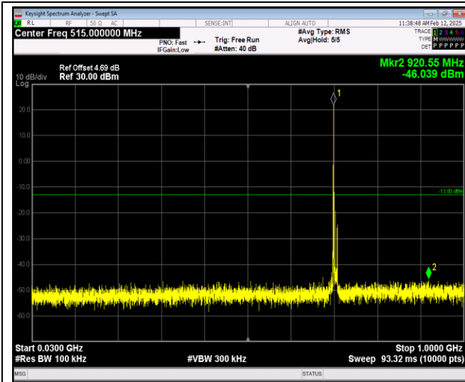
Band12-10MHz-64QAM-23060-1RB#0-Range1:30~-1000MHz
