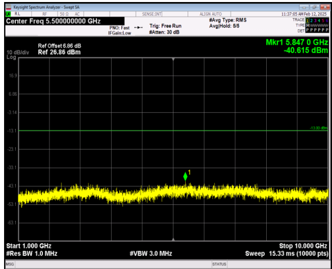
Band12-10MHz-16QAM-23095-1RB#0-Range2:1000 ~10000MHz
