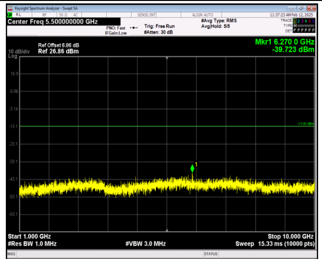
Band12-10MHz-64QAM-23095-1RB#0-Range2:1000~10000MHz
