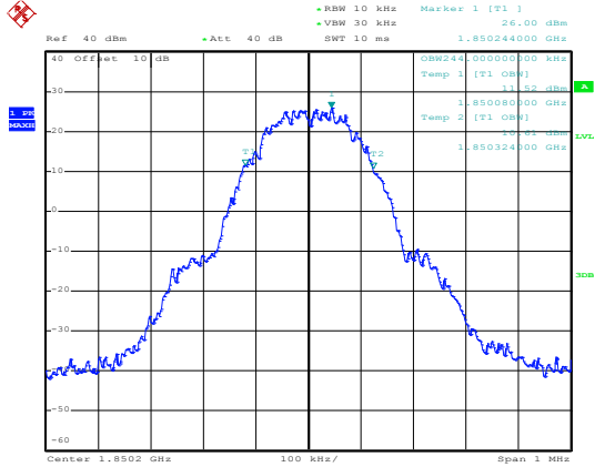
99% Occupy bandwidth
