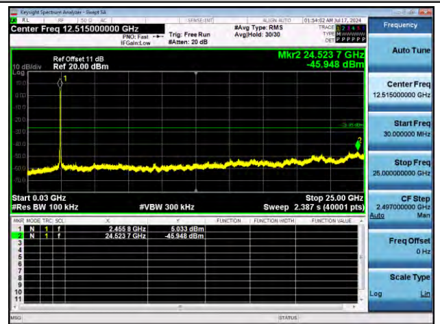
11N20SISO-Ant1-2462-30~25000-PASS
