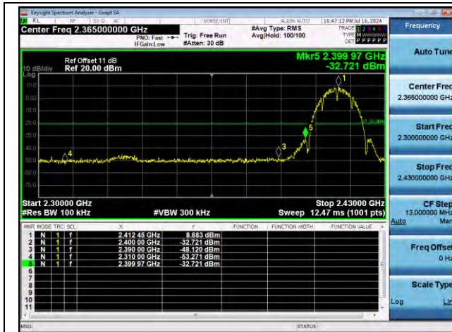
11B-Ant1-2412-PASS
