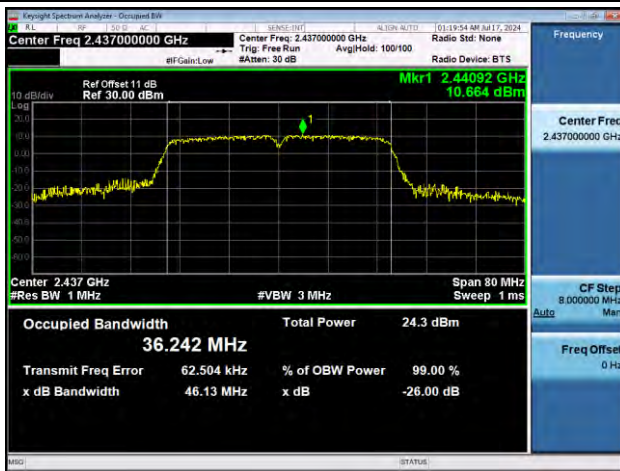
11N40SISO-Ant1-2437
