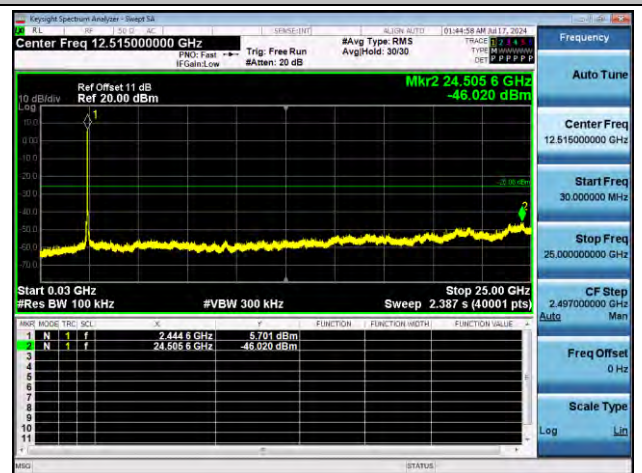
11N20SISO-Ant1-2437-30~25000-PASS
