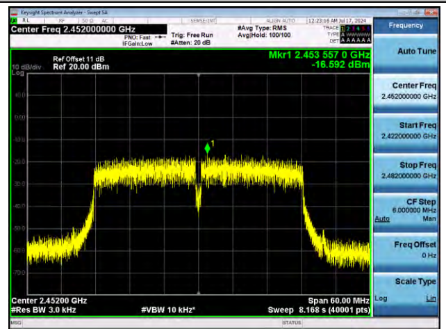
11N40SISO-Ant1-2452-PASS
