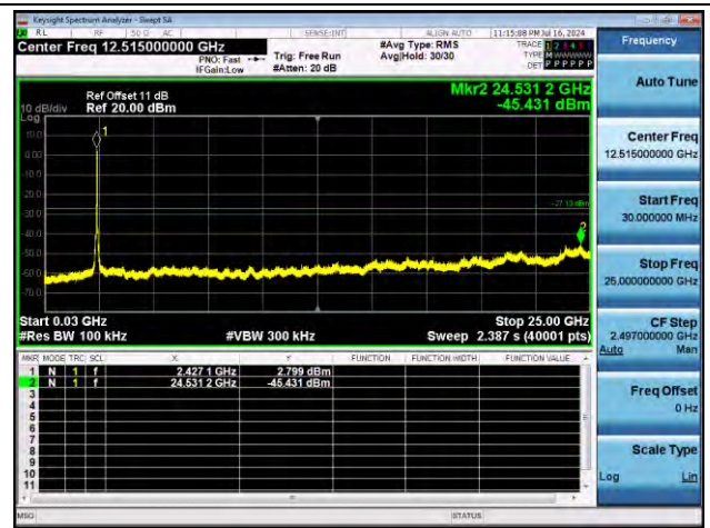
11N40SISO-Ant1-2422-30~25000-PASS
