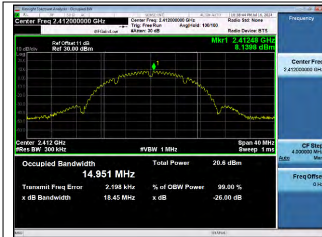
11B-Ant1-2412
