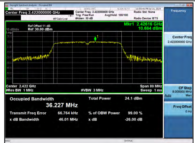
11N40SISO-Ant1-2422
