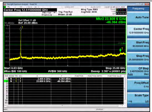
11N20SISO-Ant1-2412-30~25000-PASS
