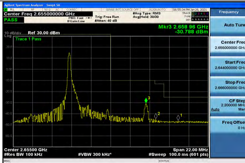
Band41-5MHz-16QAM-41215-1RB#24
