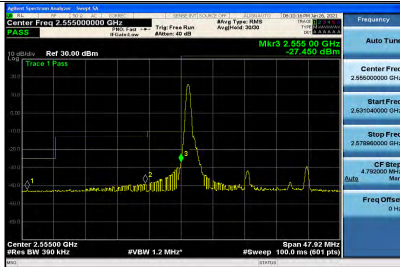
Band41-20MHz-QPSK-40340-1RB#99
