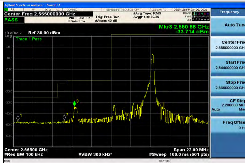
Band41-5MHz-QPSK-40265-1RB#0
