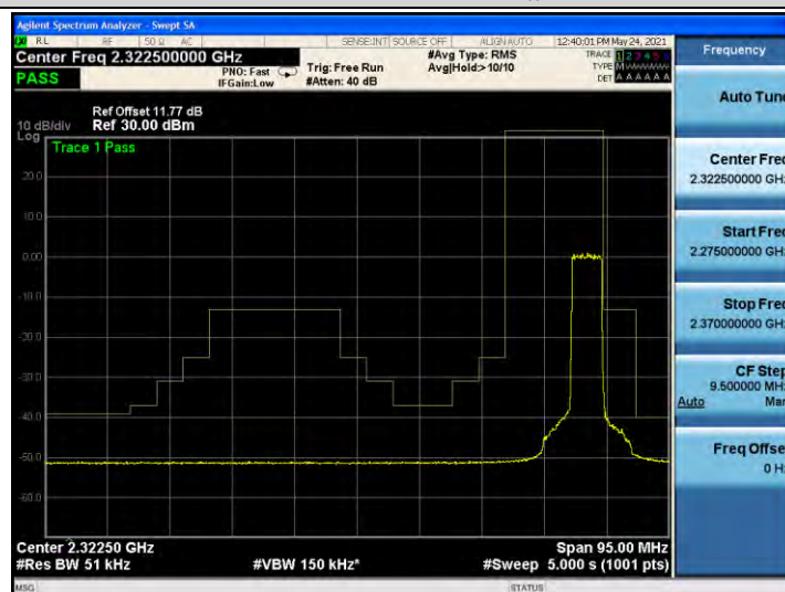
Band40-39225 25rb#0 qpsk
