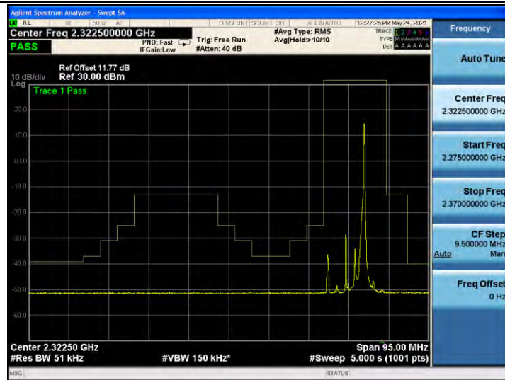
Band40-39175 25rb#0 16qam
