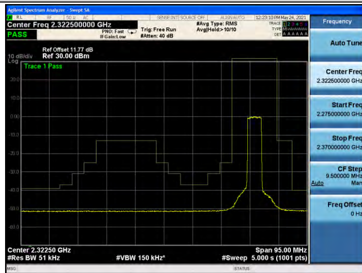
Band40-39175 25rb#0 qpsk
