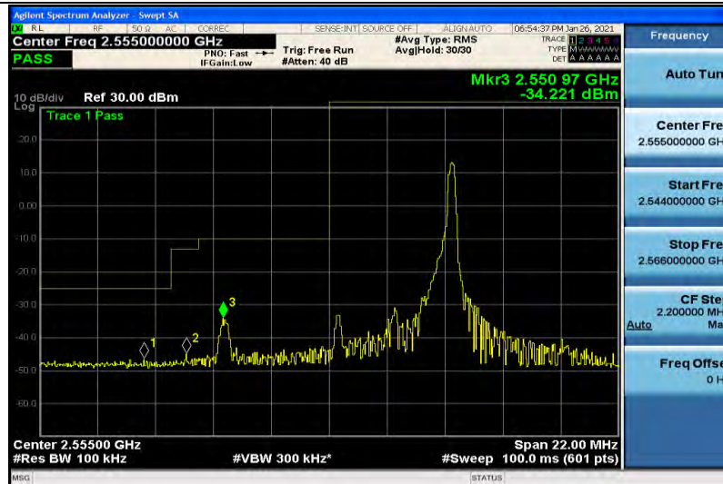
Band41-5MHz-16QAM-40265-1RB#0
