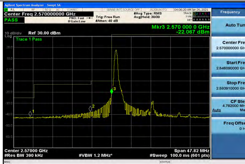
Band38-20MHz-16QAM-37850-1RB#99
