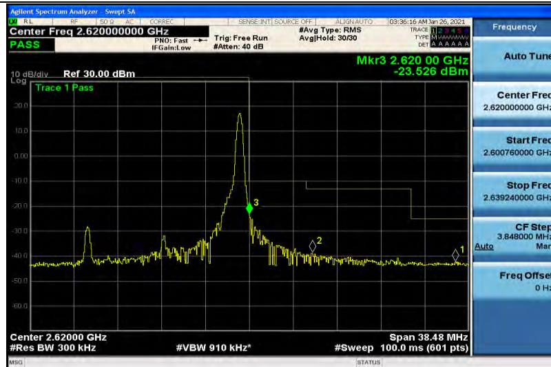
Band38-15MHz-QPSK-38175-1RB#0
