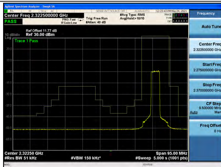
Band40-39200- 10m 1rb#0 16qam
