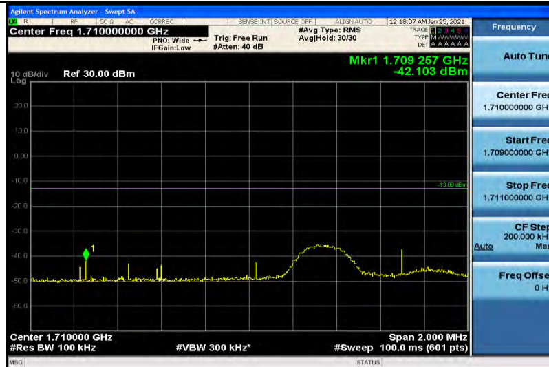
Band4-5MHz-16QAM-19975-1RB#0
