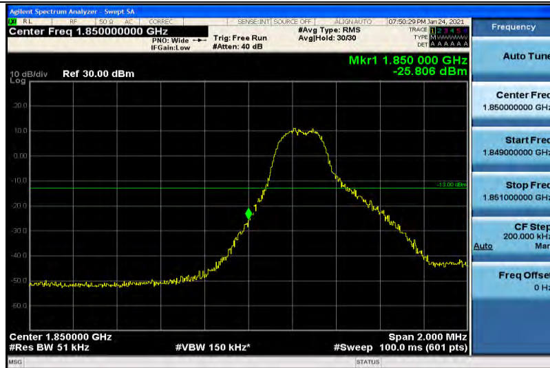
Band2-3MHz-16QAM-18615-1RB#14
