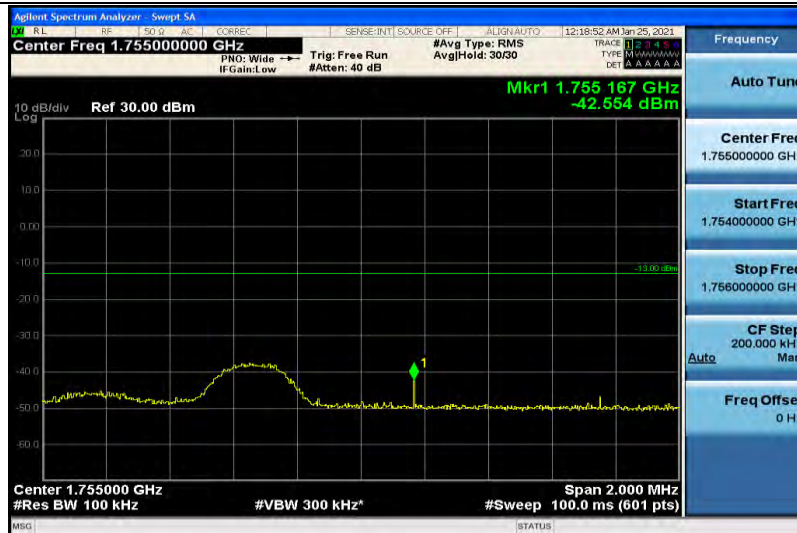
Band4-5MHz-QPSK-20375-1RB#24
